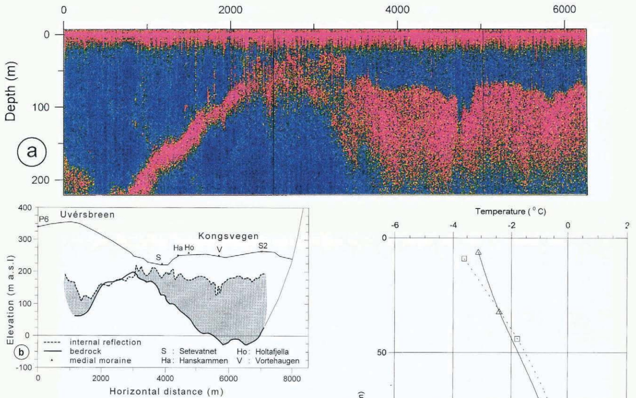
Fig. 6. Radio-echo soundings along a transverse section on Kongsvegen to Uvérsbreen from S2 to P6 (Fig. 2) and their interpretation. (a) Intensity-modulated plot of reflections of UHF radar system. (b) Interpretation of radio-echo soundings. Glacier surface elevation is based on data from Melvold (1992, personal communication, 1994) and outside the glacier from Pillewitzer (1967).
