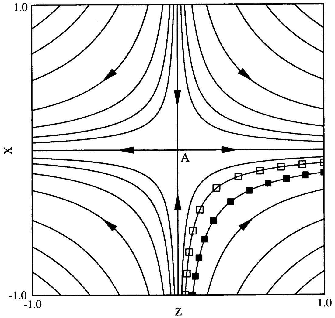
Figure 3a. Saddle of attachment surface streamlines.
