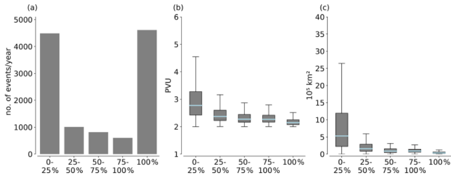
Figure 6. (a) Histogram of the percentage of air parcels in a PV cutoff experiencing decay whenever the PV cutoffs disappear on an individual isentrope (average annual number of events, 0 % corresponds to pure reabsorption, 100 % to complete diabatic decay), and (b, c) standard box plots (outliers not shown) of (b) mean PV and (c) area of the PV cutoff at the isentropic level from which it disappears for the histogram classes in (a).
