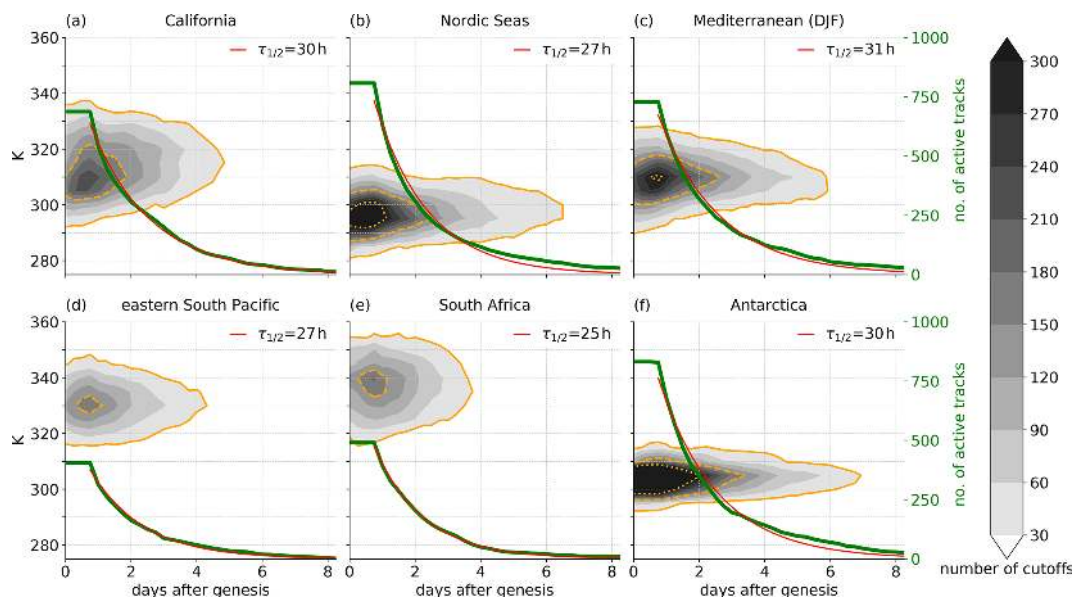
Figure 12. Number of PV cutoffs present on all isentropic levels (shading) and total number of active cutoff tracks (green curve), i.e., tracks that still persist at a certain time after genesis, and an exponential function fitted to the number of active tracks after a lifetime of one day (red curve) as a function of lifetime for PV cutoffs with genesis over the six selected regions in DJF: (a) California, (b) Nordic Seas, (c) Mediterranean, (d) eastern South Pacific, (e) South Africa, and (f) Antarctica. Values in the upper right corners correspond to PV cutoff half lives. Orange contours mark frequencies of (solid) 30, (dashed) 150, and (dotted) 300 cutoffs.
