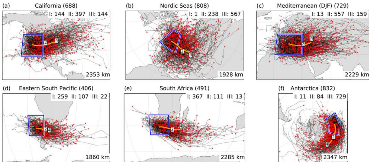
Figure 10. All tracks (black lines), lysis points (red dots), and average tracks (orange lines, including average location at days 2 and 4) of PV cutoffs with genesis over the six selected regions (blue boxes) in DJF: (a) California, (b) Nordic Seas, (c) Mediterranean, (d) eastern South Pacific, (e) South Africa, and (f) Antarctica. The average spherical distance between genesis and lysis is indicated at the bottom right of each panel.
