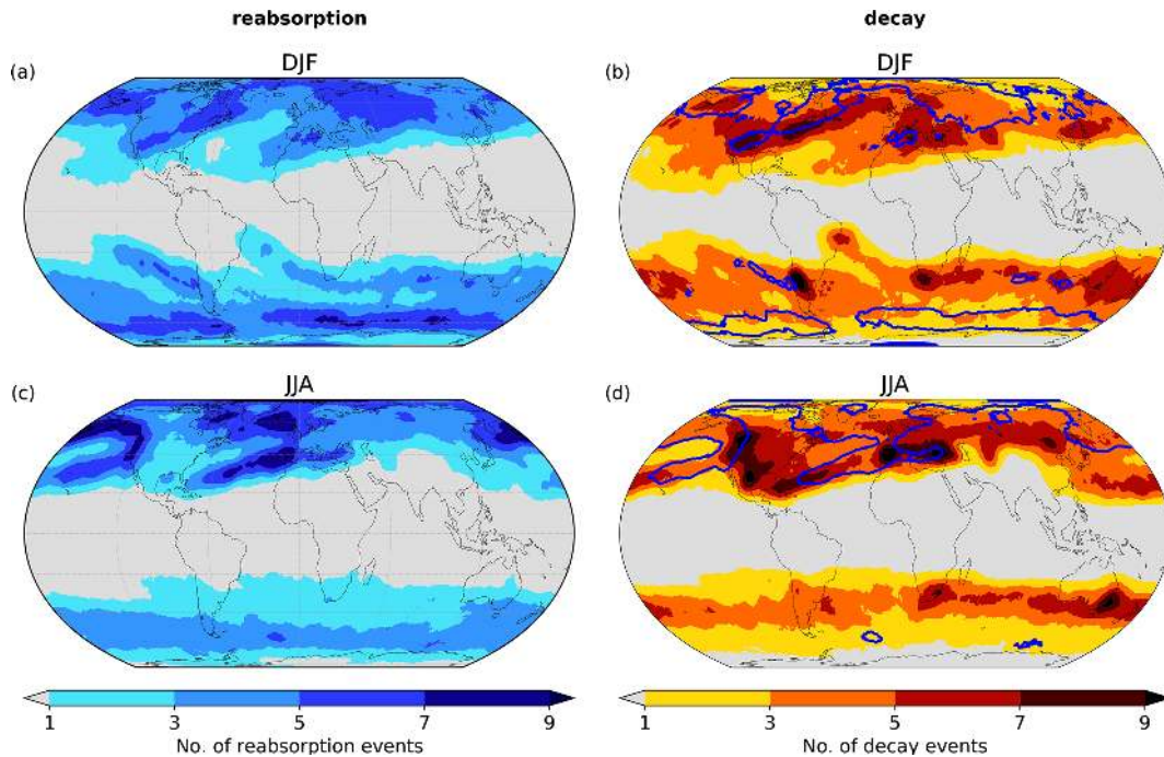
Figure 7. Average number of (a, c) reabsorption (less than 50 % decay, blue shading) and (b, d) diabatic decay (more than 50 % decay, red shading) events per season within a distance of 500 km for (a, b) DJF and (c, d) JJA. As a reference, the contour for five reabsorption events per season (blue contour) is shown (b, d).
