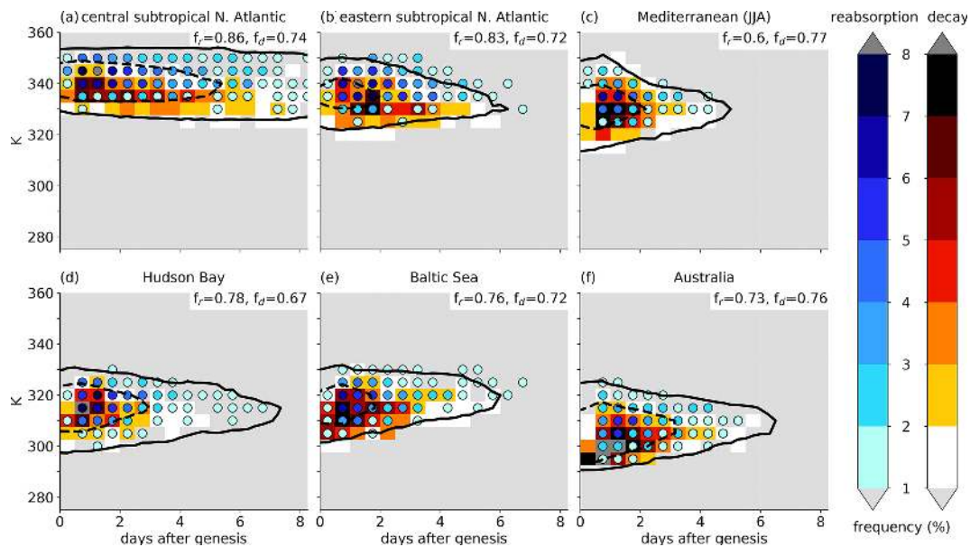
Figure 15. Same as Fig. 14 but for JJA and (a) central subtropical North Atlantic, (b) eastern subtropical North Atlantic, (c) Mediterranean, (d) Hudson Bay, (e) Baltic Sea, and (f) Australia.
