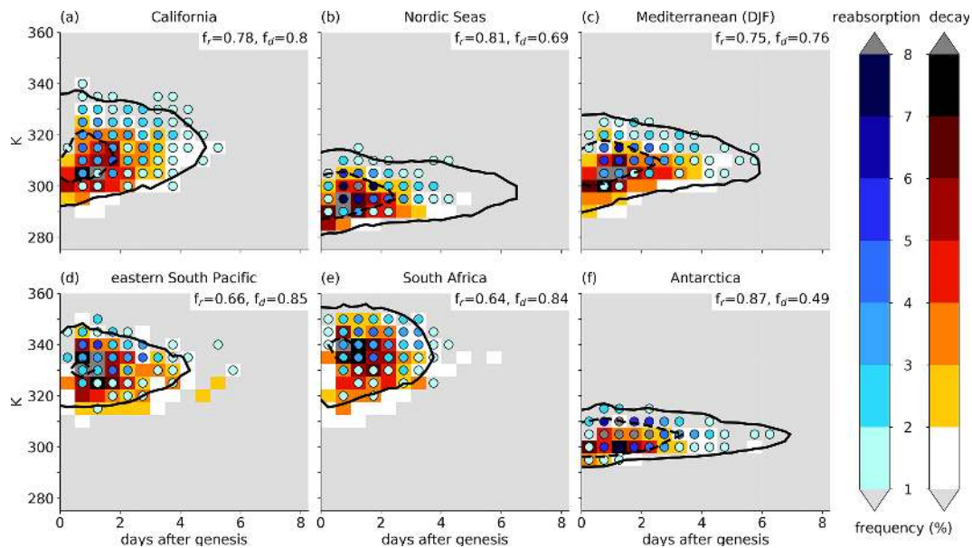
Figure 14. Relative frequency of reabsorption events (blue shaded circles, in %) and diabatic decay events (red shaded rectangles, in %) as a function of PV cutoff lifetime (binned into 12-hourly intervals) and isentropic level as well as the overall frequencies of at least one reabsorption event ( f_r ) or decay event ( f_d ) during the life cycle (numbers on top right of each panel). The climatological vertical evolution of the PV cutoffs is indicated by the black contours for (solid) 30 and (dashed) 150 cutoffs as shown in Fig. 12. Shown are the six genesis regions in DJF: (a) California, (b) Nordic Seas, (c) Mediterranean, (d) eastern South Pacific, (e) South Africa, and (f) Antarctica.
