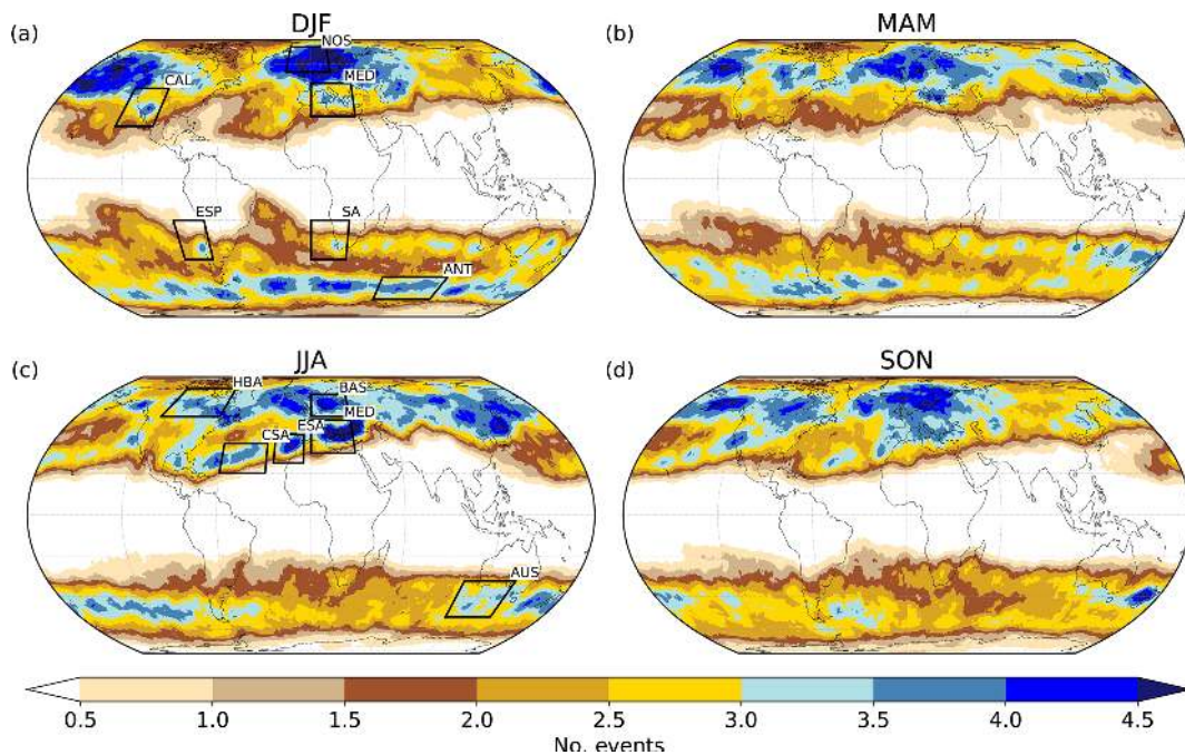
Figure 4. Seasonal average number of PV cutoff genesis events within a distance of 500 km in (a) DJF, (b) MAM, (c) JJA, and (d) SON. The location of a genesis event is determined by the center of the first PV cutoff of a track. Black boxes mark the genesis regions investigated in Sect. 4.
