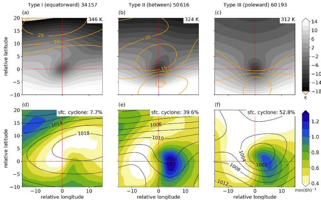
Figure 8. Cutoff-centered composites of (a–c) equivalent potential temperature at the 2PVU isosurface (shading, in K, given as difference from the domain mean value indicated at the top right of each panel) and zonal wind speed at 300 hPa (orange contours, in \text{m s}^{-1} ), and (d–f) total precipitation (shading, in \text{mm (6h)}^{-1} ) and sea level pressure (black contours, in hPa) at PV cutoff genesis, individually for (a, d) Type I, (b, e) Type II, and (c, f) Type III. The total number of tracks of each type is indicated at the top of panels (a)–(c). Additionally, the percentage of PV cutoffs linked to a surface cyclone during their life cycle is indicated for each type at the top right of panels (d)–(f).
