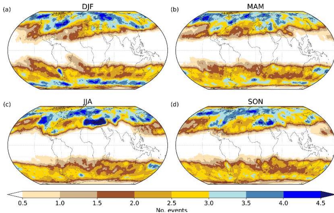
Figure 5. Seasonal average number of PV cutoff lysis events within a distance of 500 km in (a) DJF, (b) MAM, (c) JJA, and (d) SON. The location of a lysis event is determined by the center of the last PV cutoff of a track.
