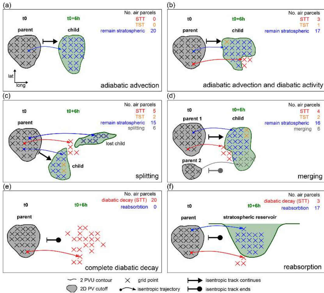
Figure 1. Schematic visualization of the tracking methodology and the associated quantification of STT, TST, diabatic decay, and reabsorption on an isentropic surface in longitude–latitude space for situations with (a) perfect adiabatic advection of the PV cutoff, (b) adiabatic advection, and the presence of diabatic processes. (c) The same as (b) but with splitting; (d) the same as (b) but with merging. (e) complete diabatic decay, and (f) reabsorption with little diabatic decay. See text for a detailed discussion.
