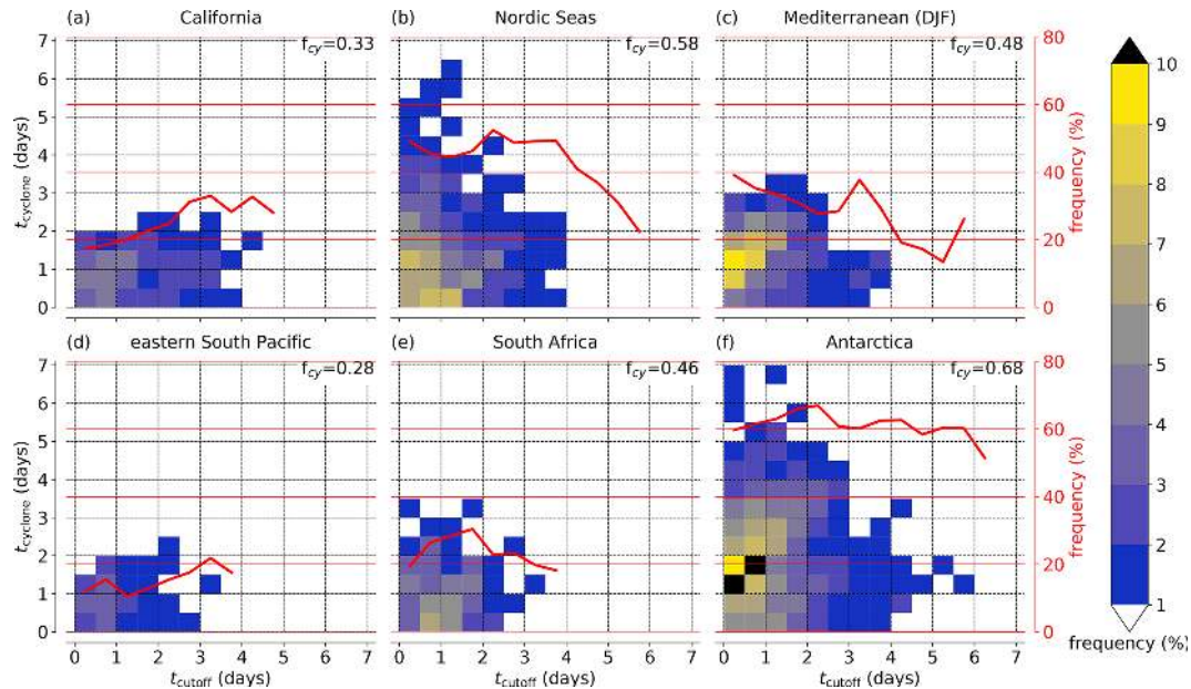
Figure 16. Relative frequencies of PV cutoffs linked to a surface cyclone (shading, in %) as a function of cutoff lifetimes ( t_{\text{cutoff}} ) on the horizontal axis and surface cyclone lifetimes ( t_{\text{cyclone}} ) on the vertical axis, binned into 12-hourly time intervals. The red contour shows the relative frequency of cutoffs linked to surface cyclones as a function of cutoff lifetime, e.g., the value at day 3 indicates the percentage of PV cutoffs with a lifetime of at least 3 d that are linked to a surface cyclone at day 3. PV cutoffs positioned in the lowermost row of the diagram are linked to a surface cyclone within 12 h after surface cyclogenesis, and PV cutoffs positioned in the leftmost column of the diagram are linked to a surface cyclone within 12 h after PV cutoff genesis. The relative frequencies of PV cutoffs with at least one link to a surface cyclone during their life cycle are indicated at the top right in each panel ( f_{\text{cy}} ). Shown are results for PV cutoffs with genesis in DJF in the regions: (a) California, (b) Nordic Seas, (c) Mediterranean, (d) eastern South Pacific, (e) South Africa, and (f) Antarctica.
