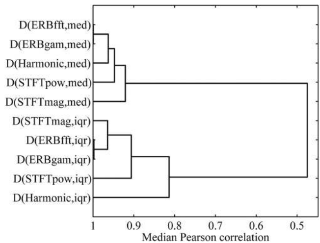
FIG. 3. Effect of the choice of input representation and descriptive statistic for time-varying descriptors on the correlation distance D between descriptors in the Timbre Toolbox. Med = median; iqr = interquartile range.
