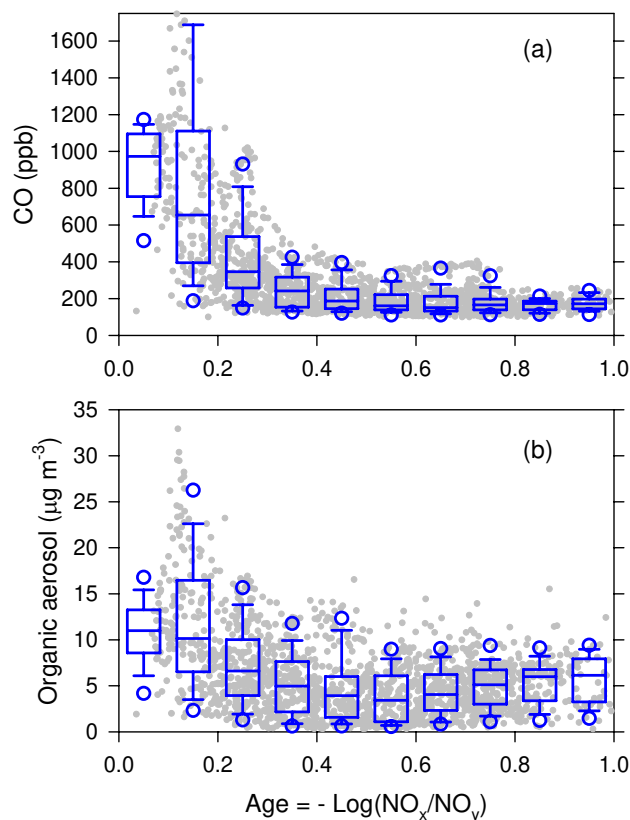
Fig. 8. (a) CO and (b) Organic aerosol concentration as a function of photochemical age. Data points are 10s average values meeting selection criteria in Table 4. Box plots give frequency distribution of data within an age bin. Box shows 75th, 50th (median) and 25th percentile of data. Caps show 90th and 10th percentiles. Circles show 95th and 5th percentiles. For clarity, bins are placed at the midpoint of age intervals. Average age in the first and last bin are 0.083 and 0.94 corresponding to \text{NO}_x/\text{NO}_y ratios of 83% and 11%, respectively.
