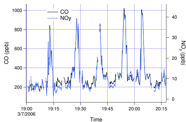
Fig. 3. Time series in UTC for CO and \text{NO}_y on flight 307a containing 5 passes through the urban plume encountered on Legs 4 and 5. Proportionality between CO and \text{NO}_y causes CO trace to be largely hidden by \text{NO}_y trace during plume passages.
