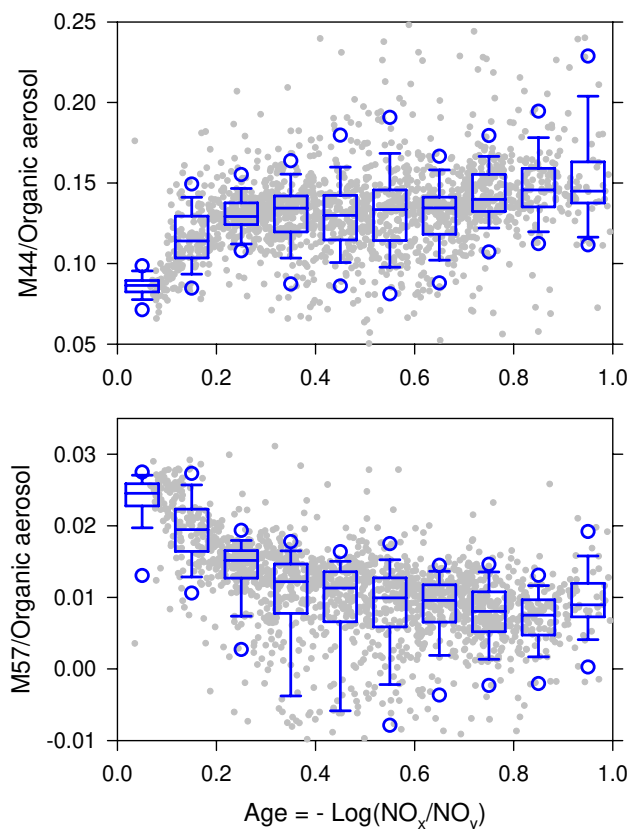
Fig. 12. Fraction of organic aerosol mass that is (a) M44 ( m/z=44 ) and (b) M57 ( m/z=57 ). Box plots have same format as Fig. 8.
