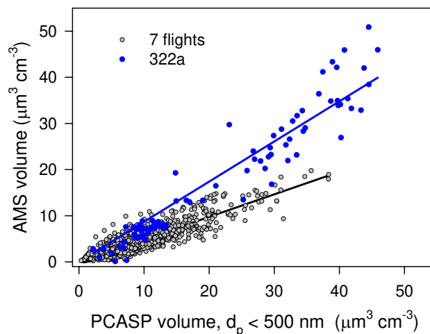
Fig. 2. Comparison of aerosol volume calculated from the AMS with that determined from the PCASP. PCASP volume includes contribution from particles with D_p < 100 nm, determined from DMA. Data points are 10 s averages that meet urban plume criteria. Lines are linear least squares fits to data constrained to pass through origin. For the first 7 flights the least squares fit has a slope of 0.49 \pm 0.004 and r^2 = 0.81 ; for the 322a flight the slope is 0.87 \pm 0.017 and r^2 = 0.91 .
