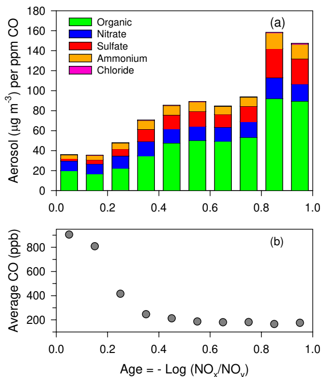
Fig. 10. (a) Aerosol concentration per ppm CO and (b) CO concentration as a function of photochemical age. For clarity, bars and data points are placed at nominal centers of the age bins, i.e. at ages 0.05, 0.15, etc. First and second age bins are closer than they appear (see Fig. 9). Speciated aerosol composition in (a) calculated from Eq. (6). Bars representing the sum of the 5 components measured by the AMS have the same magnitude as the data points in Fig. 9a.
