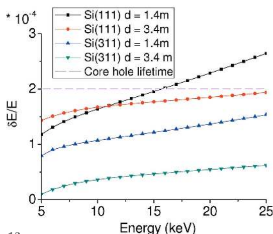
Figure 13 Energy resolution versus nominal energy, q = 0.6 m, detector at d = 1.4 m and d = 3.4 m, for Si(111) (squares and circles) and Si(311) (up and down triangles) Laue crystals.
