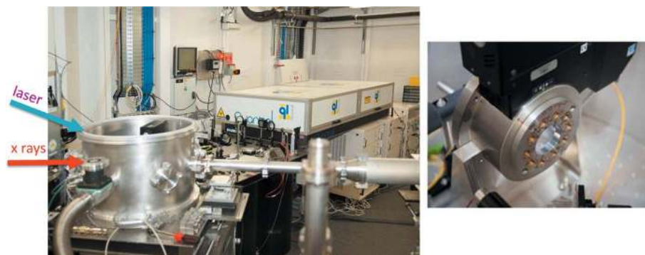
Figure 28 Left: photograph of the EDXAS_L experimental station hosting the Quantel laser from CEA (Bruyères-le-Châtel, France) and the target vacuum chamber during the dynamic compression experiment. Right: the wheel with the Fe targets.
