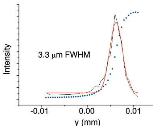
Figure 17 Knife-edge scan (blue dots) on the sample position along the horizontal direction. A Gaussian fit (red line) to the derivative (black line) yields a spot size of 3.3 μm FWHM.
