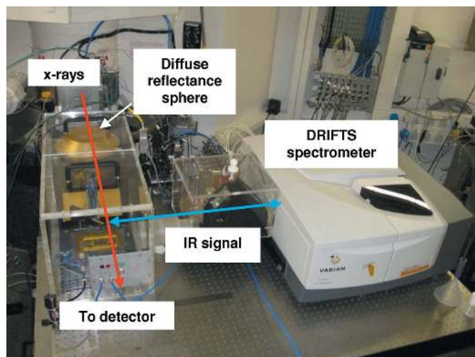
Figure 26 Photograph of the XAS/DRIFT/MS facility in EDXAS_L.
