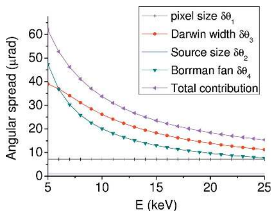
Figure 12 Angular contributions to the energy resolution for a 200 \mu\text{m} -thick Si(111) Laue crystal focusing at q = 0.6 m with a detector at d = 3.4 m.
