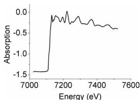
Figure 18 Example of Fe K -edge EXAFS of a standard 4 μm-thick polycrystalline Fe foil placed in a diamond anvil cell. The dimensions of the focal spot are those illustrated in Fig. 17.
