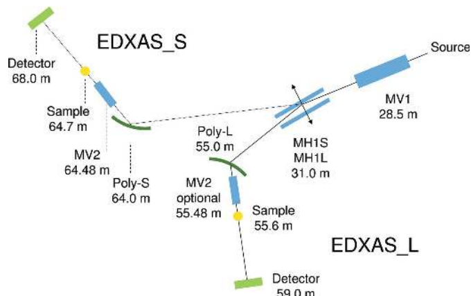
Figure 4 Beamline ID24 at the ESRF: the new design features two branches, EDXAS_S and EDXAS_L. Mirrors are in blue, polychromators in green, samples in yellow and detectors in light green. Acronyms MH1S, MH1L, MV1, MV2 are explained in the text.
