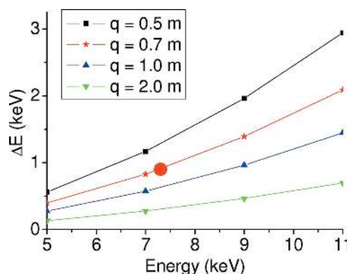
Figure 8 Full spectral range \Delta E diffracted by a Si(111) polychromator as a function of central energy E_0 , from equations (1) and (2), calculated for branch EDXAS_S ( L = 50 mm and p = 29.7 m). The red dot marks the measured \Delta E value at the Fe K -edge, with q = 0.7 m.
