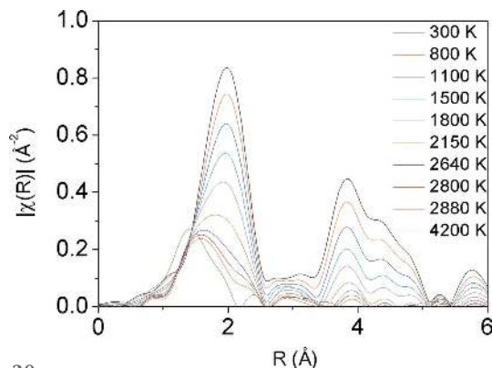
Figure 30 Evolution of the magnitude of Fourier transforms of Ni K -edge EXAFS during in situ laser heating of pure Ni foil to above the melting temperature, at 66 GPa. The most intense spectrum corresponds to Ni at ambient T . As T increases, the intensity of the peaks decreases and the first shell becomes asymmetric.
