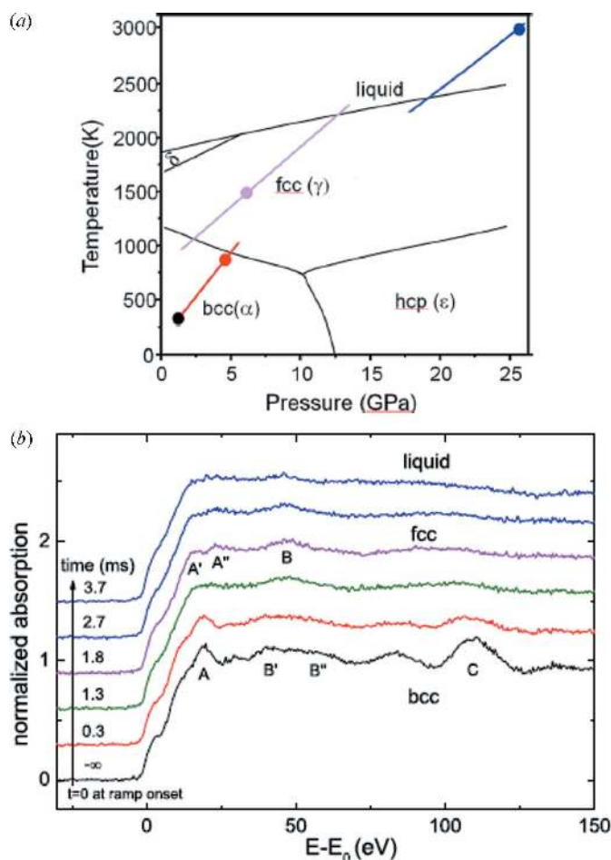
Figure 31 (a) Iron phase diagram and isochoic path for the bcc, fcc and liquid phases. The dots indicate roughly estimated P, T conditions for the black, red, pink and blue spectra shown in (b). (b) Sequence of Fe K -edge XANES selected during a fast ohmic ramp. The bottom spectrum (black) has been collected before the start. Acquisition time is 25 \mu s per spectrum. [Reprinted with permission from Marini et al. (2014). Copyright 2014, AIP Publishing LLC.]
