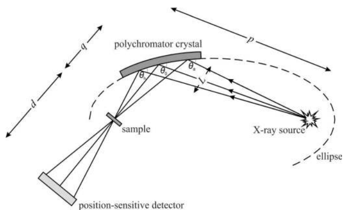
Figure 7 Principle of operation of the energy-dispersive XAS spectrometer. On beamline ID24, the X-ray source in this figure is a demagnified image of the undulator source ( i.e. secondary source).
