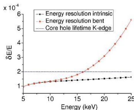
Figure 11 Energy resolution versus nominal energy E_0 , q = 0.7 m, detector at d = 3.3 m for a Si(111) Bragg crystal.
