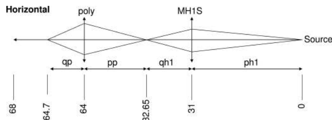
Figure 15 Optical scheme of the EDXAS_S branch in the horizontal plane.
