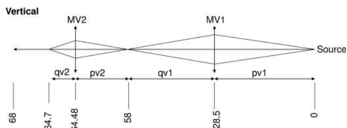
Figure 5 Optical scheme of the EDXAS_S branch in the vertical plane.
