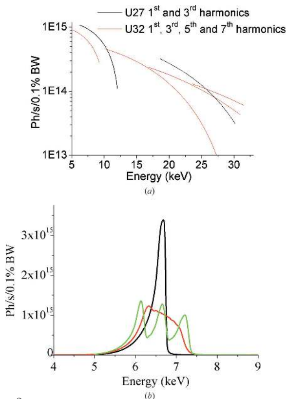
Figure 3 (a) Photons \text{s}^{-1} (0.1% bandwidth) ^{-1} at 200 mA delivered by 1.6 m U32/U27 undulators over the beamline energy range 5–28 keV. (b) Effect of tapering. Using three tapered U27 undulators, an energy range of \sim 1 keV can be achieved at 7 keV. Black: the three U27 undulators are at gap = 11.5 mm, no taper. Green: gaps = 11.0 mm, 11.7 mm and 12.5 mm, no taper. Red: gap = 11.75 mm using a linear taper of 1.5 mm.
