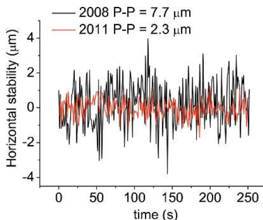
Figure 22 Movements of the beam in the horizontal plane, measured on the focal spot, as a function of time. A factor three reduction in PP amplitude is achieved with the new supports.
