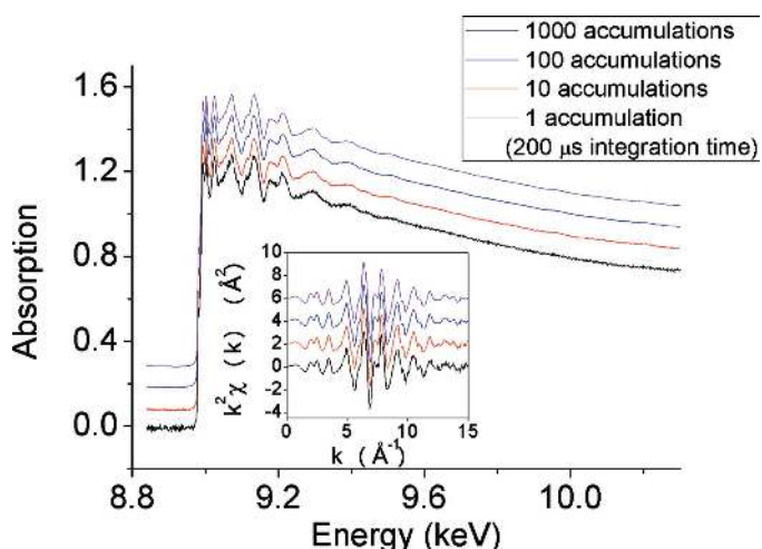
Figure 23 Sequence of Cu K -edge EXAFS acquired with the new Hamamatsu chip. From bottom to top: average of 1, 10, 100, 1000 accumulations of 200 \mu\text{s} each. The accumulated curves are offset from the single accumulation for clarity. The inset shows the k^2\chi(k) signals. Taken from Kantor et al. (2014).
