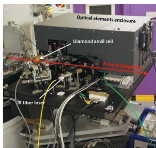
Figure 24 Schematic drawing (left) and photograph (right) of the in situ laser-heating facility for high-pressure studies with the DAC. 1: DAC; 2: high-power IR laser beams; 3: emitted radiation from hot sample; 4: spectrometer; 5: CCD video camera and microscope; 6: green laser for Raman spectroscopy.
