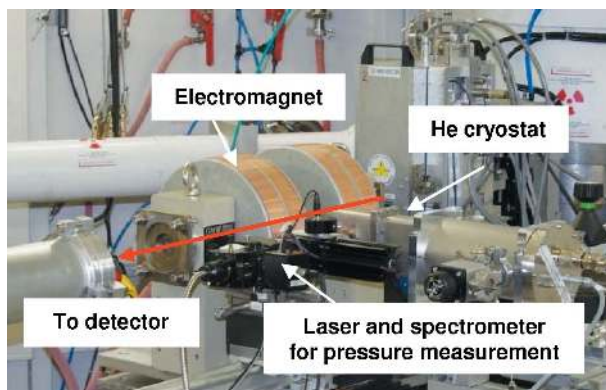
Figure 27 The XMCD facility for high-pressure and low-temperature studies.
