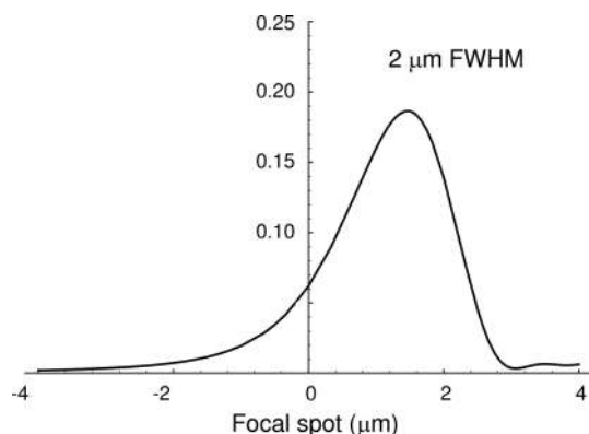
Figure 16 Contribution to the focal spot size for a Si(111) crystal at 7 keV with p = 30 m and q = 1 m.
