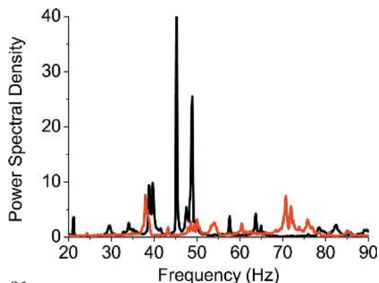
Figure 21 Power spectral density of beam instabilities in the vertical plane, measured on the focal spot, in 2008 (black) and 2011 (red). The reduction in the amplitude of vibrations between 30 and 50 Hz is visible.
