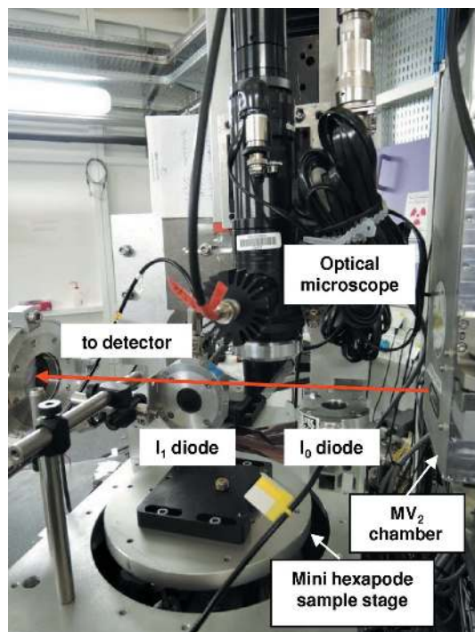
Figure 25 Photograph of the micro-XAS facility on EDXAS_S.
