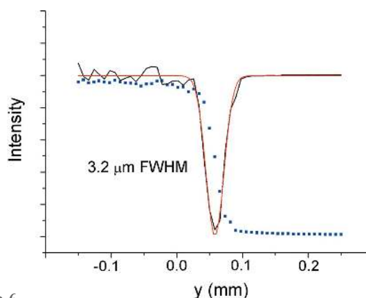
Figure 6 Knife-edge scan (blue dots) on the sample position along the vertical direction. A Gaussian fit (red line) to the derivative (black line) yields a spot size of 3.2 \mu\text{m} FWHM.
