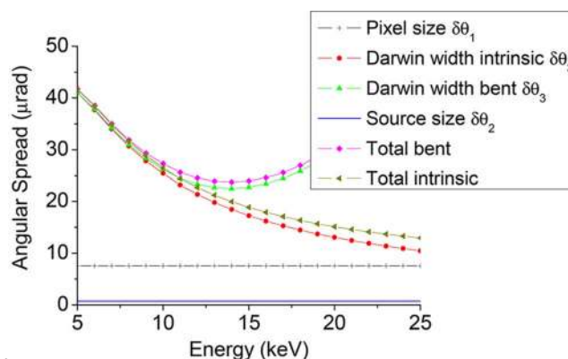
Figure 10 Angular contribution to the energy resolution versus nominal energy E_0 , q = 0.7 m, detector at d = 3.3 m for a Si(111) Bragg crystal.
