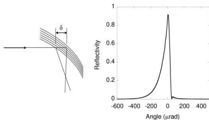
Figure 9 Left: schematic effect of X-ray penetration in a curved crystal. Right: simulation of the diffraction profile deformation of Si(111) crystal at 15 keV due to a 3 m radius of curvature.
