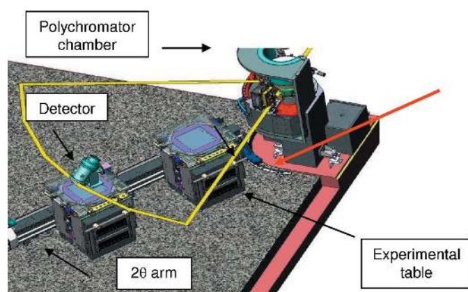
Figure 20 Schematic drawing of the experimental hutch on branch EDXAS_L. The granite floor covers the full surface of the hutch. The experimental table, the detector support and the 2\theta arm are moved on airpads mounted on granite chassis. The 2\theta arm is used only as a guide. The red arrow indicates the X-ray propagation direction.
