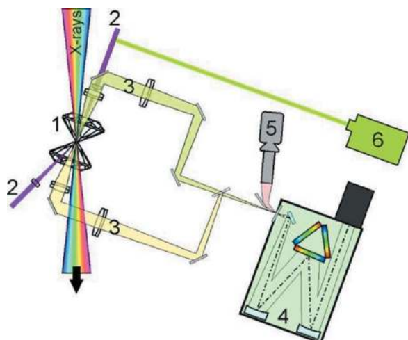
Figure 24 Schematic drawing (left) and photograph (right) of the in situ laser-heating facility for high-pressure studies with the DAC. 1: DAC; 2: high-power IR laser beams; 3: emitted radiation from hot sample; 4: spectrometer; 5: CCD video camera and microscope; 6: green laser for Raman spectroscopy.
