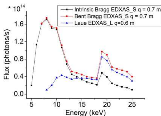
Figure 14 Flux on sample for a Si(111) crystal. Squares: EDXAS_S, Bragg geometry (intrinsic Darwin width), q = 0.7 m. Circles: EDXAS_S, Bragg geometry (bent Darwin width), q = 0.7 m. Triangles: EDXAS_L, Laue geometry, q = 0.6 m. Between 13 and 18 keV, only the two U32 undulators contribute to the flux.
