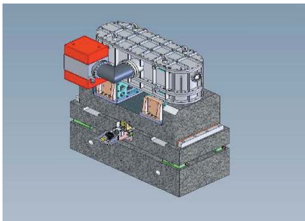
Figure 19 The design of the new support for MV1 features three successive granite blocks and highly accurate and ultra-stable mirror positioning systems.
