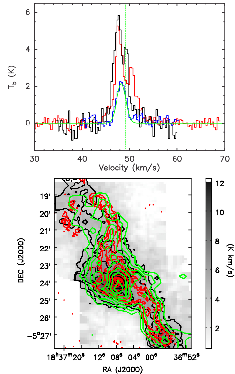
Figure 17. Upper panel: The spectra of ^{13}\text{CO} (1-0) and ^{13}\text{CO} (2-1) at the continuum peak are shown in black and red, respectively. The spectrum of \text{C}^{18}\text{O} (1-0) averaged over an region of 1' \times 1' is shown in blue. The Gaussian fit of \text{C}^{18}\text{O} (1-0) is shown in green. The green dashed vertical line marks the systemic velocity of 49 \text{ km s}^{-1} . Lower panel: Integrated intensity ( 47\text{-}50 \text{ km s}^{-1} ) map of ^{13}\text{CO} (2-1) is shown in gray scale and black contours. The contour levels are from 30% to 90% in steps of 10% of the peak value ( 12.9 \text{ K km s}^{-1} ). Integrated intensity ( 47\text{-}50 \text{ km s}^{-1} ) map of \text{C}^{18}\text{O} (1-0) is shown in green contours. The contour levels are from 30% to 90% in steps of 10% of the peak value ( 6.4 \text{ K km s}^{-1} ). The SCUBA-2 850 \mu\text{m} continuum emission in the R2 data reduction is shown in red contours. The contour levels are [0.03, 0.05, 0.1, 0.2, 0.4, 0.6, 0.8] \times 1.40 \text{ Jy beam}^{-1} .
