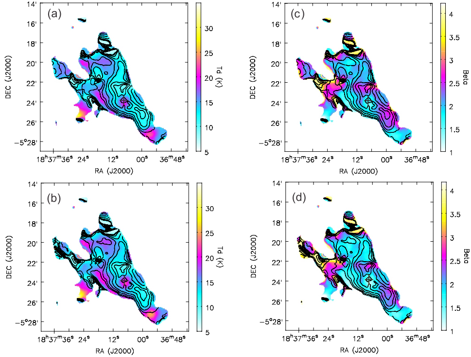
Figure 7. (a). The dust temperature map in the SED fit with free \beta using the Herschel data only is shown in color image. The 250\ \mu\text{m} optical depth is shown in contours. The contour levels are [0.03, 0.05, 0.1, 0.2, 0.4, 0.6, 0.8] \times 0.0282 (b). The dust temperature map in the SED fit with free \beta using both the Herschel and SCUBA-2 data is shown in color image. The 250\ \mu\text{m} optical depth is shown in contours. The contour levels are [0.03, 0.05, 0.1, 0.2, 0.4, 0.6, 0.8] \times 0.0211 (c). The \beta map in the SED fit with free \beta using the Herschel data only is shown in color image. The 250\ \mu\text{m} optical depth is shown in contours. The contour levels are the same as in panel a. (d). The \beta map in the SED fit with free \beta using both the Herschel and SCUBA-2 data is shown in color image. The 250\ \mu\text{m} optical depth is shown in contours. The contour levels are the same as in panel b. The crosses in the four panels mark the position of the most massive clump.
