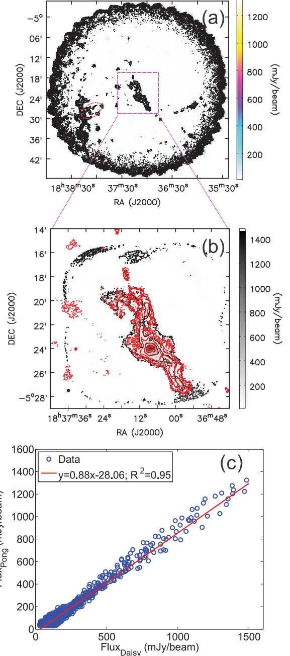
Figure A4. (a). The Pong1800 SCUBA-2 850 \mu\text{m} map. The contours are [0.03, 0.05, 0.1, 0.2, 0.4, 0.6, 0.8] \times 1.32 \text{ Jy beam}^{-1} . The red dashed ellipse marks the position of the infrared bubble shown in Figure 12. (b). Close-up of the Pong1800 SCUBA-2 850 \mu\text{m} map in the Daisy map region is shown in red contours. The gray scale image and black contours show the CV Daisy map. The contour levels are [0.05, 0.1, 0.2, 0.4, 0.6, 0.8] \times 1.48 \text{ Jy beam}^{-1} . (c). Comparison of flux in the Daisy map with flux in the Pong map for pixels with S/N > 3 . The red line shows the linear fit.
