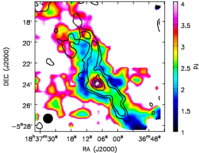
Figure 18. The CO gas depletion factor is shown as color image. The column density map from SED fits with Herschel and combined Planck and SCUBA-2 850 \mu\text{m} data in R2 is shown in contours. The contour levels are [0.15, 0.2, 0.4, 0.6, 0.8] \times 2.76 \times 10^{23} \text{ cm}^{-2} .
