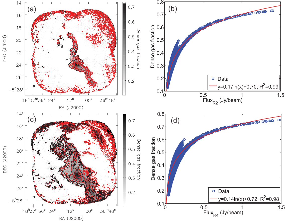
Figure 10. (a). The dense gas fraction in R2 reduction is shown in gray-scale and red contours. The contour levels are [0.2, 0.3, 0.4, 0.5, 0.6, 0.7]. The 850\ \mu\text{m} continuum emission in R2 reduction is shown in black contours. The contour levels are the same as in the lower panel of Figure A2. (b). The dense gas fraction vs. the 850\ \mu\text{m} continuum flux density in the R2 reduction. The red line shows the logarithmic function fit toward the pixels with flux density larger than 200\ \text{mJy beam}^{-1} in the SCUBA-2 image. (c). The dense gas fraction in R4 reduction is shown in gray-scale and red contours. The contour levels are [0.2, 0.3, 0.4, 0.5, 0.6, 0.7]. The 850\ \mu\text{m} continuum emission in R4 reduction is shown in black contours. The contour levels are the same as in Figure A3b. (d). The dense gas fraction vs. the 850\ \mu\text{m} continuum flux density in the R4 reduction. The red line shows the logarithmic function fit toward the pixels with flux density larger than 300\ \text{mJy beam}^{-1} in the SCUBA-2 image.
