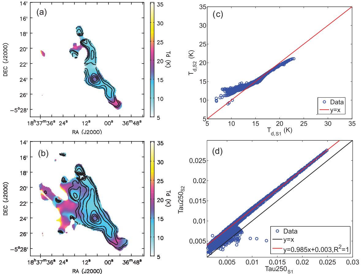
Figure 5. (a). The dust temperature map in the S1 SED fit is shown in color-scale image. The 250 \mu\text{m} optical depth is shown in contours. The contour levels are [0.03, 0.05, 0.1, 0.2, 0.4, 0.6, 0.8] \times 0.0270 (b). The dust temperature map in the S2 SED fit is shown in color-scale image. The 250 \mu\text{m} optical depth is shown in contours. The contour levels are [0.03, 0.05, 0.1, 0.2, 0.4, 0.6, 0.8] \times 0.0275 (c). Comparison of the dust temperature values in S1 and S2 . Only data points with S/N > 5 in SCUBA-2 map are considered. (d). Comparison of the 250 \mu\text{m} optical depth in S1 and S2 . Only data points with S/N > 5 in SCUBA-2 map are considered. The red line shows the linear fit toward the data points with 250 \mu\text{m} optical depth larger than 0.01 in S4 .
