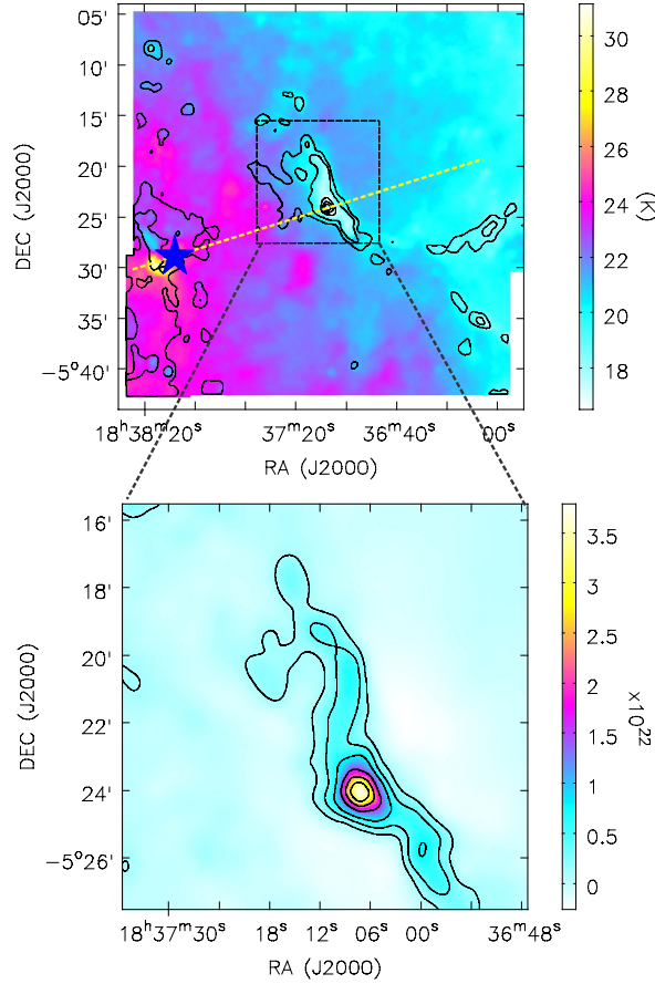
Figure A1. Upper panel: From Herschel data, column density contours overlaid on a dust temperature color image. The contour levels are [0.15, 0.2, 0.4, 0.6, 0.8] \times 4.8 \times 10^{22} cm -2 . The blue star marks the position of the infrared bubble shown in Figure 12. The yellow dashed line marks the direction along which the cuts in Figure 13 were made. Lower panel: Close-up of column density map from Herschel data over the SCUBA-2 mapped region. The large scale emission in Herschel bands was filtered out. The contour levels are [0.03, 0.1, 0.2, 0.4, 0.6, 0.8] \times 3.8 \times 10^{22} cm -2 .
