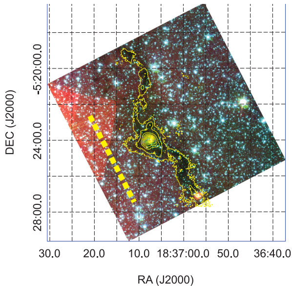
Figure 4. Spitzer/IRAC three color ( 3.6 \mu\text{m} in blue, 4.5 \mu\text{m} in green, and 8 \mu\text{m} in red) composite image of PGCC G26.53+0.71. The yellow contours represent the SCUBA-2 850 \mu\text{m} continuum emission with filtering out scales of >200'' . The contour levels are [0.03, 0.05, 0.1, 0.2, 0.4, 0.6, 0.8] \times 1.38 \text{ Jy beam}^{-1} . The yellow dashed line shows the direction of the Galactic Plane.
