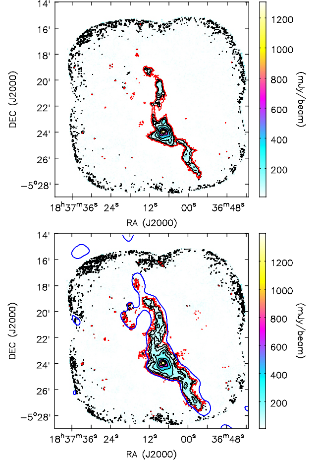
Figure A2. Upper panel: The SCUBA-2 850 \mu m continuum emission in the R1 data reduction for G26. The contour levels are [0.03, 0.05, 0.1, 0.2, 0.4, 0.6, 0.8] \times 1.35 Jy beam -1 . Lower panel: The SCUBA-2 850 \mu m continuum emission in the R2 data reduction. The contour levels are [0.03, 0.05, 0.1, 0.2, 0.4, 0.6, 0.8] \times 1.40 Jy beam -1 . The red contour in both panels shows the S/N level of 3.
