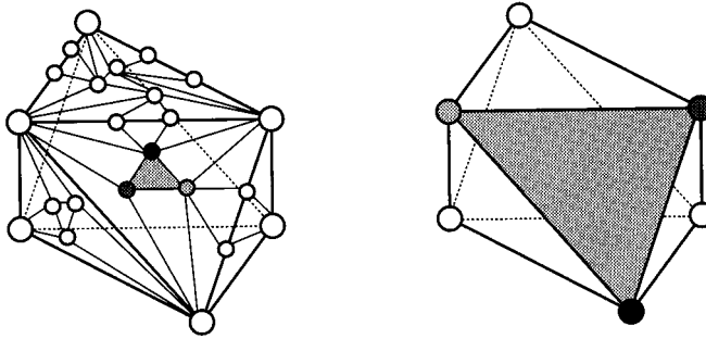
FIG. 7. A simplex and its carrier.
