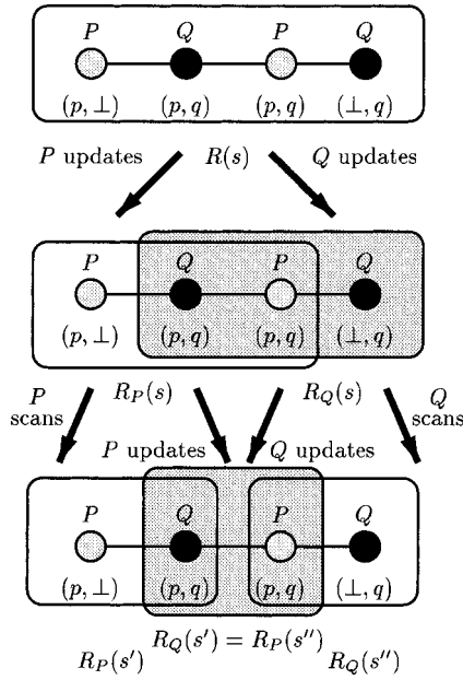
FIG. 27. Connectivity of reachable complexes.
