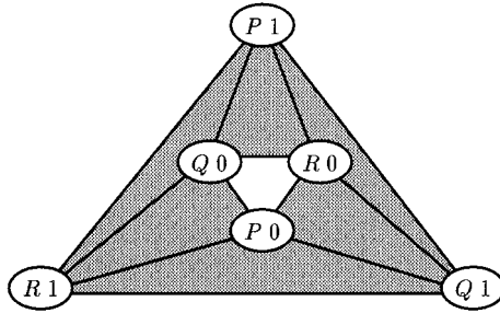
FIG. 36. Reduced renaming output complex \mathcal{O}^2 .
