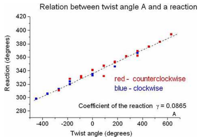
Figure 2. The relation between a twist angle A and a reaction.
