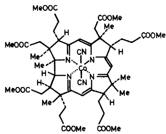
Heptamethyl bisnorneocobyrinate
