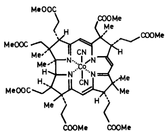
Heptamethyl bisnorcobyrinate
