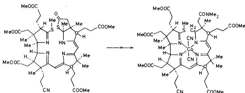
S-Methyldithiocyanocorrigenolide
