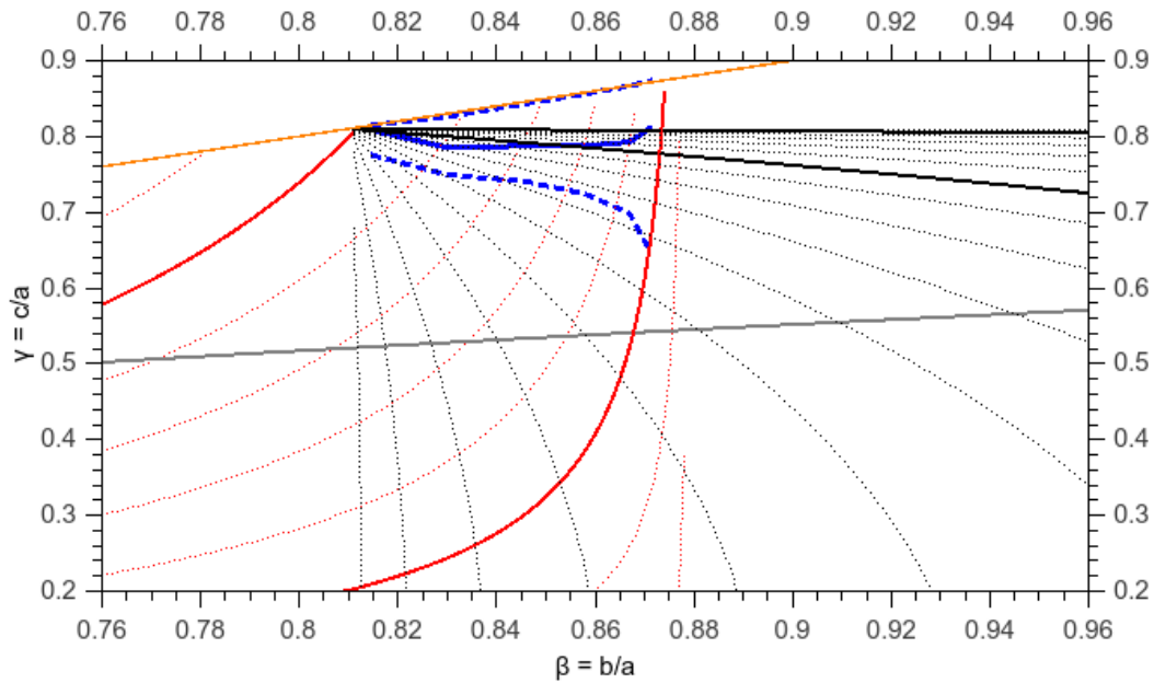
FIGURE 13. Relation between \beta = b/a and \gamma = c/a combining eq. A2 (black dotted lines – as in Fig. 11) and eq. A4 (red dotted lines – as in Fig. 12). Blue curve is the intersection between the black and red lines for each value of \theta and the uncertainties (dotted blue lines – which depends on the determination of \beta^0 and \Delta m ). The orange line is the value for \beta = \gamma while the grey line represents the relation for \beta and \gamma for the Jacobi shape. For \theta between 55 and 80°, defined by the black and red full lines, there is no intersection between the blue and grey lines, meaning that there is no Jacobi solution for VS2.
