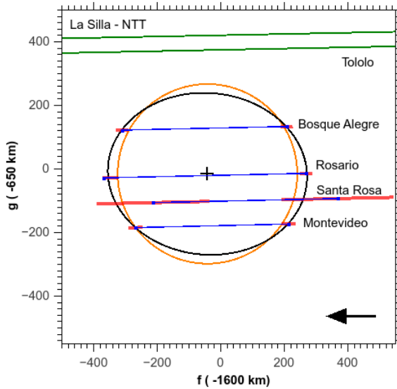
FIGURE 8. Occultation chords (blue) and their uncertainties (red) from the multi-chord event of November 2014 with the best elliptical fit (black). The offsets in both axis are with respect to ephemeride positions obtained using JPL#30 and DE431. The arrow shows the direction of the shadow motion and the green lines represent the two closest sites from where there were no detection of the occultation (see Table 5). The equivalent circle (that has the same area as the ellipse) is shown in orange with a diameter of 564.8 km.
