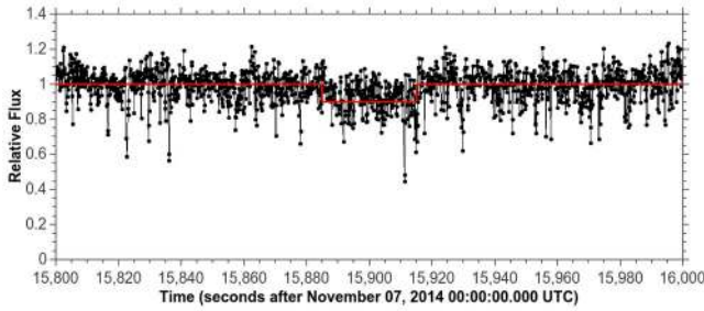
FIGURE 10. Light curve from the multi-chord stellar occultation of November 07, 2014 obtained at La Silla/NTT. All the flux drops in the curve are due to the star being too close to the edge of the CCD or being influenced by the bad row of pixels in the center of the CCD. Note the relative flux drop of 0.09 that happens between instants 15885 s and 15915 s, fitted using a square well model, represented by the red line.
