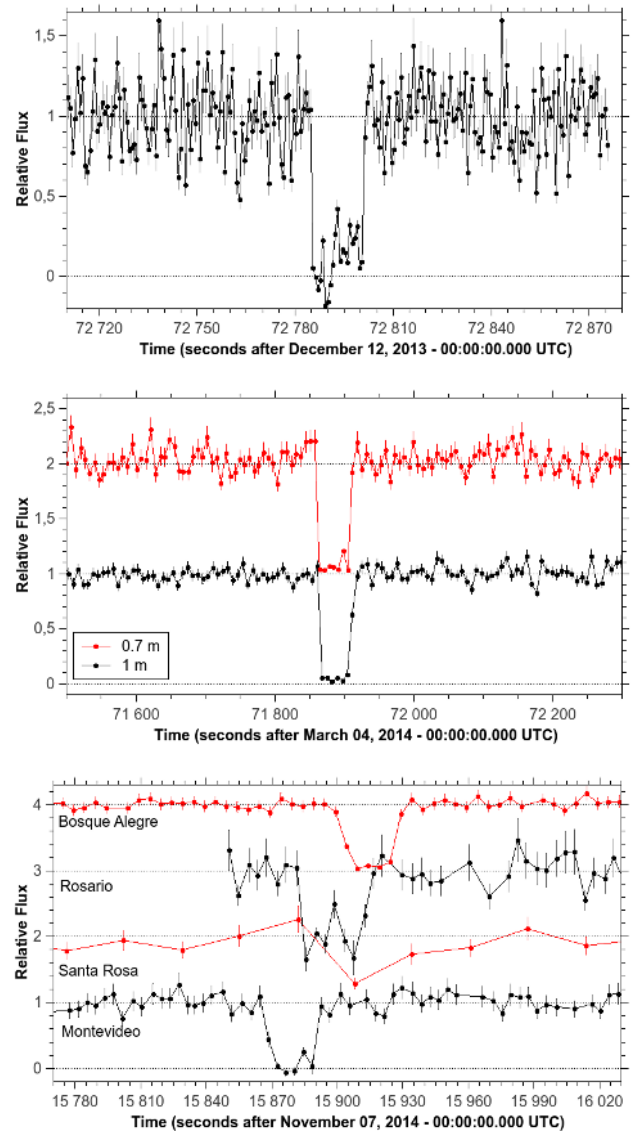
FIGURE 5. Normalized light curves of the positive detections of the stellar occultations – see Tables 4 and 5 for sites details. TOP: single-chord event in December 12, 2013; CENTER: single-chord event in March 04, 2014, showing the detection with the two telescopes at the same site; BOTTOM: multi-chord event on November 2014. Chords are shifted in flux for better visualization. Vertical lines are the uncertainties in photometry for each point.
