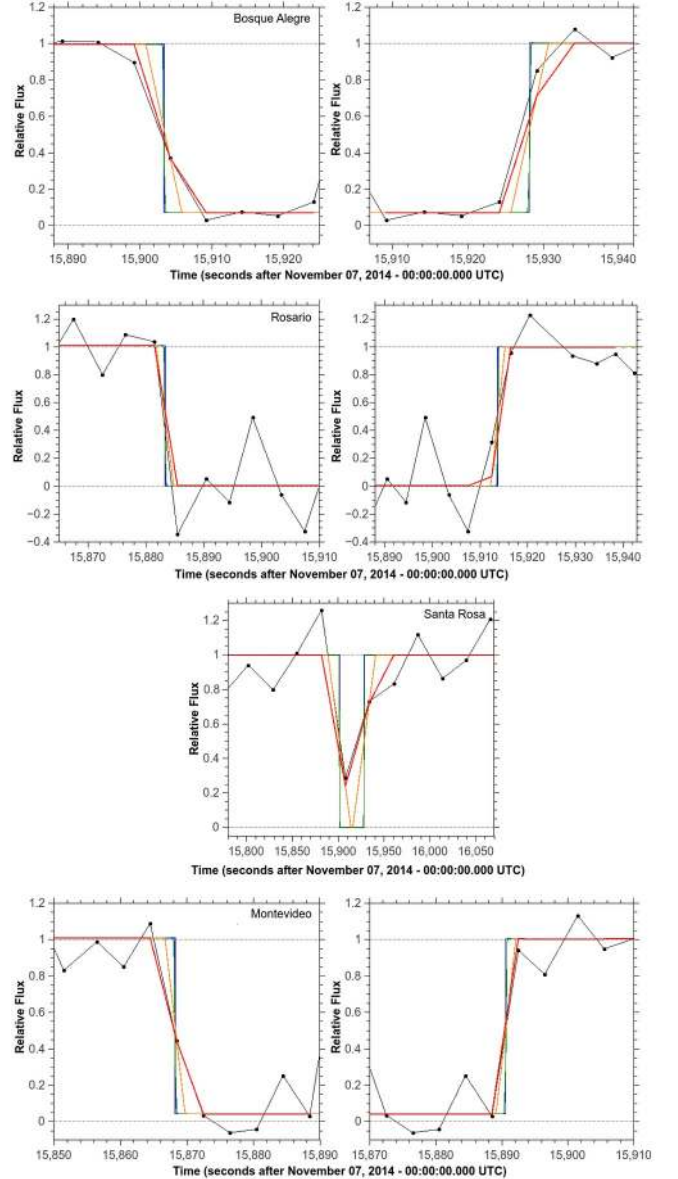
FIGURE 7. Best fit for the star disappearance (left) and reappearance (right) instants of the multi-chord event of November 07, 2014 – see Table 5 for sites details. From top to bottom: Bosque Alegre, Rosario, Santa Rosa, and Montevideo. Line colors are the same as in Fig. 6.
