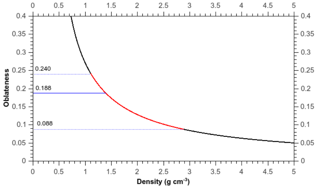
FIGURE 14. Relation between and density for a Maclaurin object with rotation period of 7.4175285 hours (black line). The oblateness obtained for VS2 (blue horizontal full and dotted lines) gives limits for the minimum value of the density of 1.4 \text{ g cm}^{-3} . Blue dotted lines represent the values considering the uncertainties in a and b . Red line is the interval between the limits.
