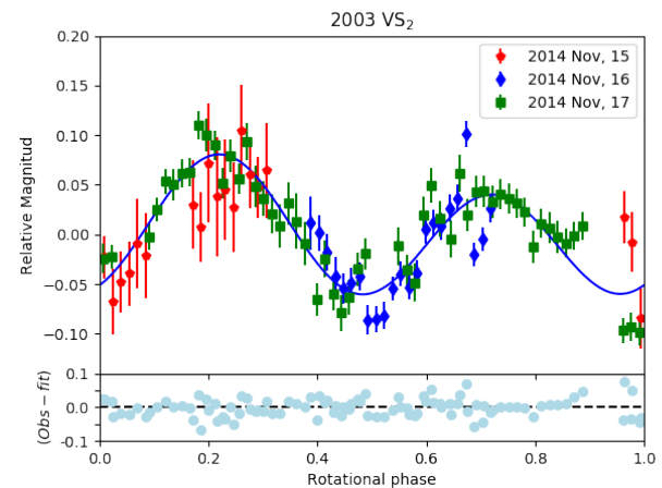
FIGURE 4. Rotational light curve for VS2 obtained on November 15 (in red), 16 (in blue) and 17 (in green), 2014 at Sierra Nevada Observatory (see text for details) just a few days after the occultation. Light blue dots on the bottom panel show the residuals between the observed points and the fit (blue line). The estimated rotational phase for the November 2014 stellar occultation is near one of the brightness maxima. We used the occultation date as the zero phase date.
