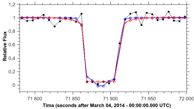
FIGURE 9. Light curve from the single-chord stellar occultation of March 04, 2014 obtained at Wise Observatory (black) and the two models for the isothermic pure nitrogen (red) and a Pluto-like (blue) atmospheres within a 3\sigma limit.
