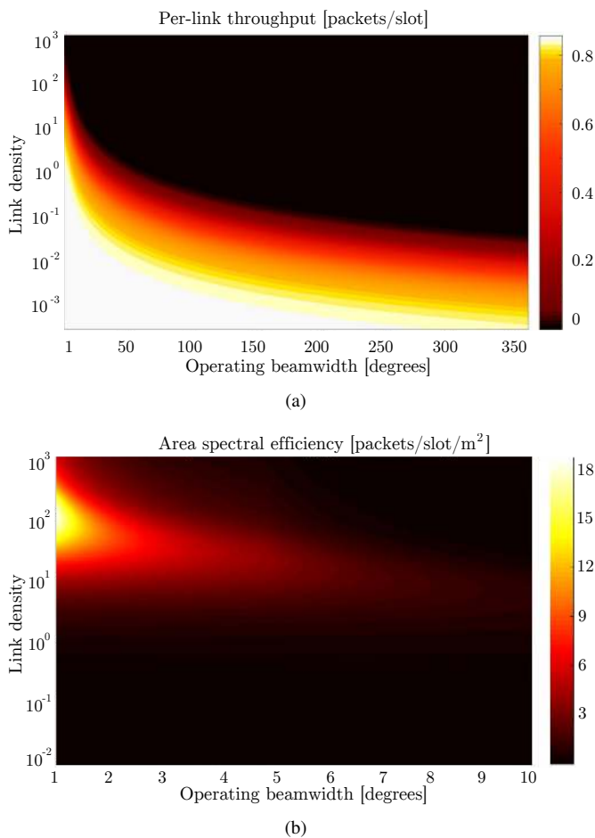
Fig. 6. Achievable regions of (a) per-link throughput and (b) area spectral efficiency of slotted ALOHA with \rho_\alpha = 1 .
