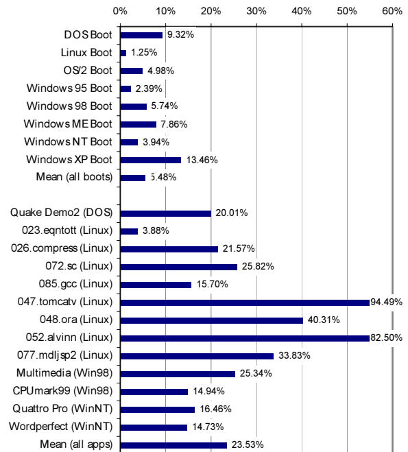
Figure 3: Degradation Caused By No Alias Hardware
