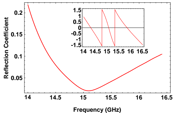
Figure 4: Magnitude of the reflection coefficient of the HOM couplers (shown inset is the corresponding phase)
