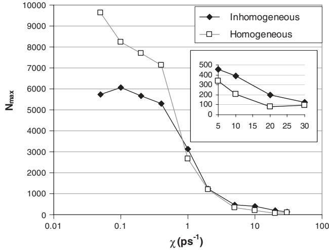
Figure 13. The peak number of (mostly unstable) defects measured during the cascade evolution as a function of electron-phonon coupling ( \chi = \beta_p/M_i ). At high coupling, the use of an inhomogeneous evolving electronic temperature distribution is seen to enhance the degree of ionic mixing. The cascade is prolonged by the feedback of energy from electrons to ions. As in figure 12 above, no simple interpretation of the data for \chi \lesssim 1 \text{ ps}^{-1} is possible. (From Rutherford and Duffy [9].)
