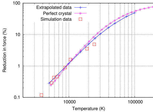
Figure 20. The percentage reduction in the average magnitude of the attractive electronic force with rising temperature in a TDTB model. Data shown are: (Red) squares, reduction in the force found in cascade simulations up to 50 keV PKA energy, plotted against the best-fit temperature to the excited electronic system. (Purple) circles, the calculated reduction in the force based on the temperature dependence of the bond orders in a perfect crystal. (Blue) crosses, the change in force found for an electronic temperature in a static system distorted to reflect the ionic positions during cascade simulations. (From Race et al. [14].)
