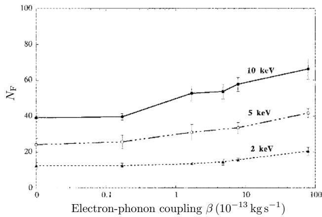
Figure 11. The number of Frenkel pairs produced in cascades with various PKA energies as a function of electron-phonon coupling strength. (From Gao et al. [84].)
