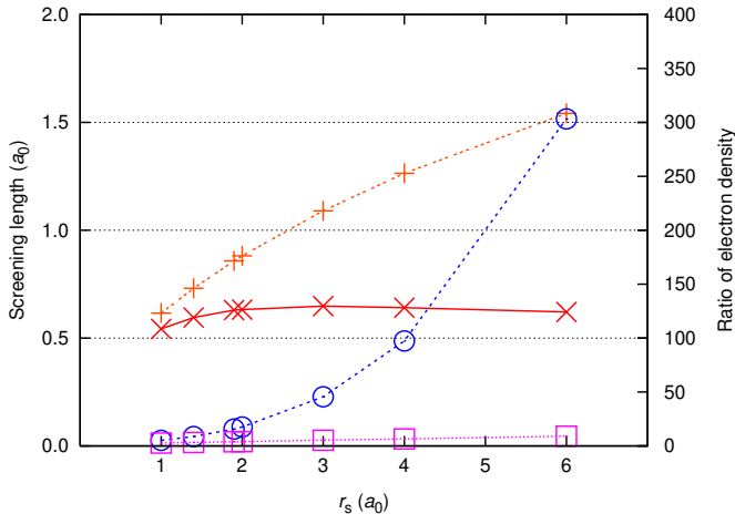
Figure 4. Calculated results for a proton in a free-electron gas of varying density (parameterized by the one electron radius r_s = (3/4\pi n_e)^{1/3} ). The screening length is indicated for linear response (orange vertical crosses) and non-linear DFT calculations (red diagonal crosses). Distances are given in atomic units, a_0 = 0.529 \text{ \AA} . On the right-hand axis are plotted the ratio of the charge density at the proton position to the background density for linear response (purple squares) and non-linear DFT calculations (blue circles). (Data from Almbladh et al. [60].)
