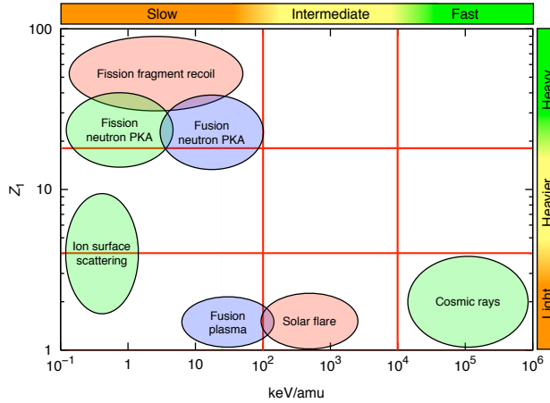
Figure 1. The classification of electronic stopping behaviour into various regimes based on projectile atomic number and kinetic energy per atomic mass unit. A sample of applications is indicated on the chart according to their corresponding regimes.
