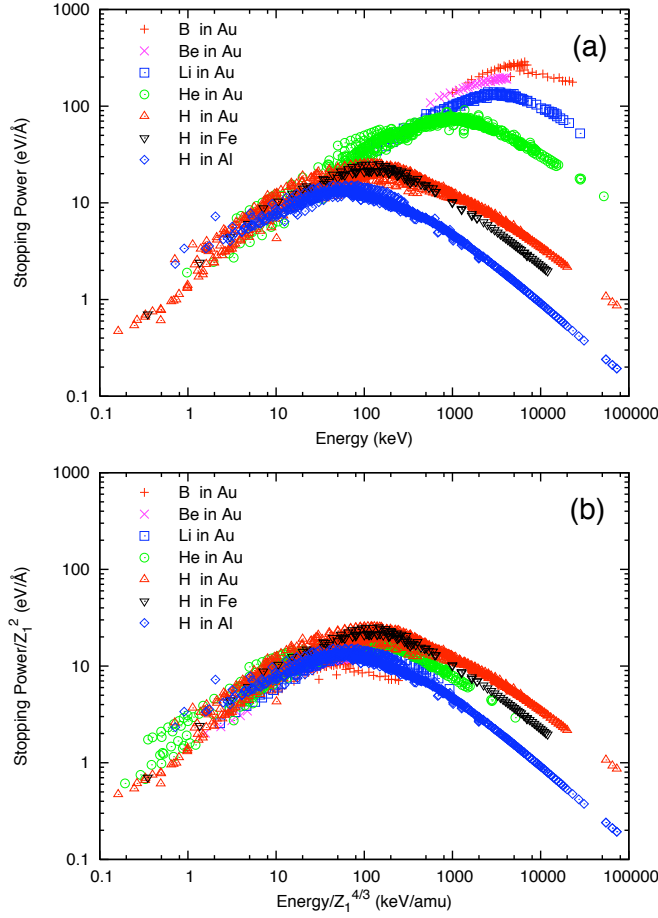
Figure 8. A demonstration of how simple scaling relationships (b) can capture much of the behaviour of the electronic stopping power (a) for a variety of projectile and target combinations. The scaling of stopping power by 1/Z_1^2 is informed by the pre-factor in the fast particle stopping theories (6), (8) and (18) and the normalisation of the particle velocity by 1/Z_1^{2/3} is suggested by the Thomas-Fermi scaling of electronic velocities. (Data are from the database of Paul [25].)
