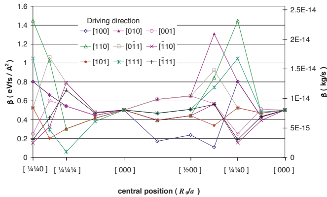
Figure 17. As figure 16 except that the oscillating ion is moved away from its lattice site to the positions indicated and oscillated at a fixed frequency, \Omega = 1 \text{ rad fs}^{-1} . The damping for an off-site oscillator is anisotropic and is plotted for a selection of directions of oscillation. A rich structure emerges, with a variation in \beta of an order of magnitude with direction and position. (From Mason et al. [147].)
