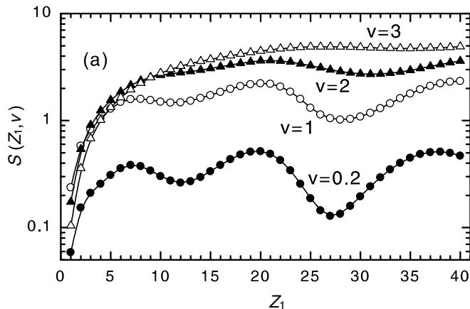
Figure 7. The Z_1 -structure in the stopping power for bare ions in a free electron gas of density equivalent to that in carbon at several projectile velocities (given in units of v_0 ). (From Arista [63].)
