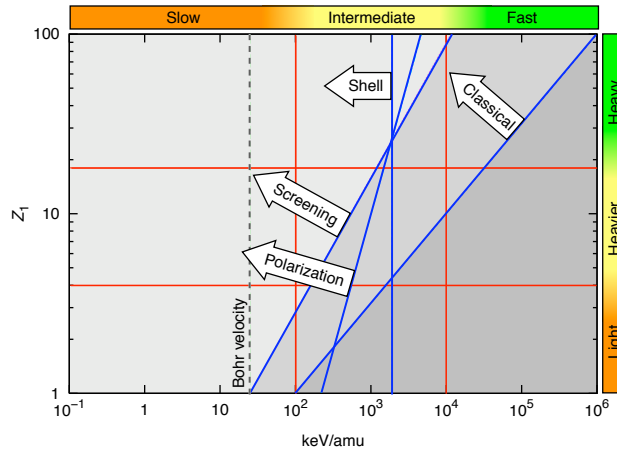
Figure 3. The projectile kinetic energy and atomic number regimes of electronic stopping theory in an iron target ( Z_2 = 26 ) showing order of magnitude thresholds for various effects and corrections. Bohr’s classical threshold v \lesssim 2Z_1 v_0 is shown, along with the thresholds for screening ( v \lesssim Z_1^{2/3} v_0 ) and Barkas (polarization) ( v \lesssim (Z_1 Z_2)^{1/3} v_0 ) effects. The velocity at which shell effects become important ( v \lesssim Z_2^{2/3} v_0 ) and the Bohr velocity, v_0 , below which the projectile ion will have very low charge with many bound states are also indicated. (After Sigmund [39].)
