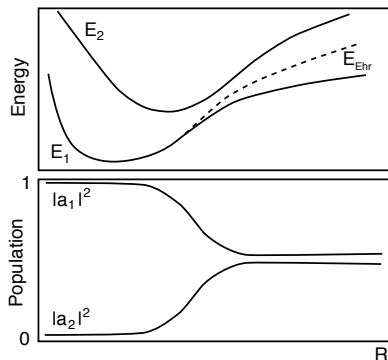
Figure 14. A schematic representation of the variation of the energies E_{1,2} and occupation probabilities |a_{1,2}|^2 of a pair of energy eigenstates as function of an ionic coordinate R . We are assuming that R is changing sufficiently quickly that non-adiabatic transitions within the system are stimulated. As the probabilities evolve, the potential energy surface E_{\text{Ehr}} traversed by the Ehrenfest system is a weighted average, representative of neither eigenstate. (After [129].)
