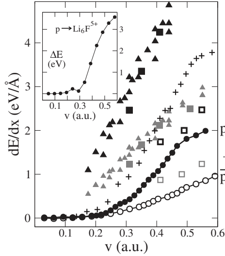
Figure 15. Electronic stopping power dE/dx as a function of particle velocity from time-dependent DFT simulations of channelling in LiF. The results for protons are shown as filled circles, anti-protons as empty circles. The crosses show results for protons when extra basis states are added along the channelling particle’s path. The insert and other data are discussed in [138]. (From Pruneda et al. [138].)
