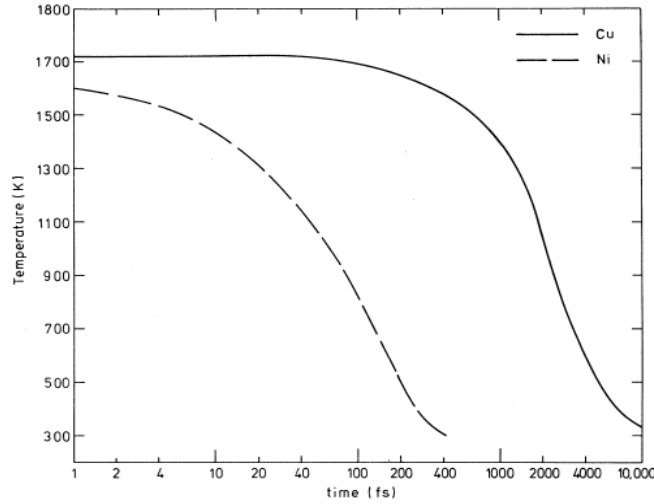
Figure 9. The evolution of the ionic temperature given by the coupled equations (46) and (47) for values of g_p , the electron-phonon coupling constant, for Cu and Ni. (From Finnis et al. [83].)
