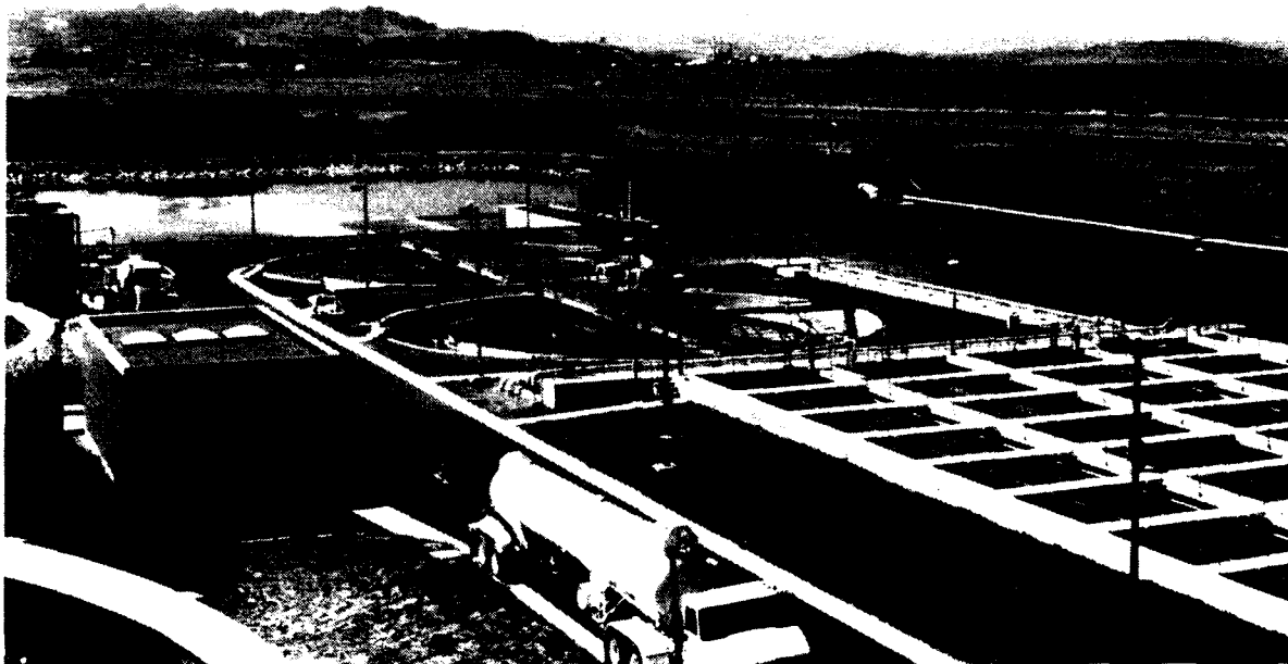
Figure A1. Overview of the Elk River trickling filter/solids contact treatment plant at Eureka, CA. Primary sedimentation tanks are in the right foreground. The L-shaped aerated solids contact tank can be seen between the primary and secondary clarifiers. Secondary clarifiers are in the center, and the effluent holding pond is behind the clarifiers. (Source: Brown and Caldwell Consulting Engineers. Used with permission.)
