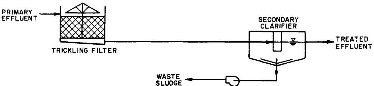
D. TRICKLING FILTER PROCESS
