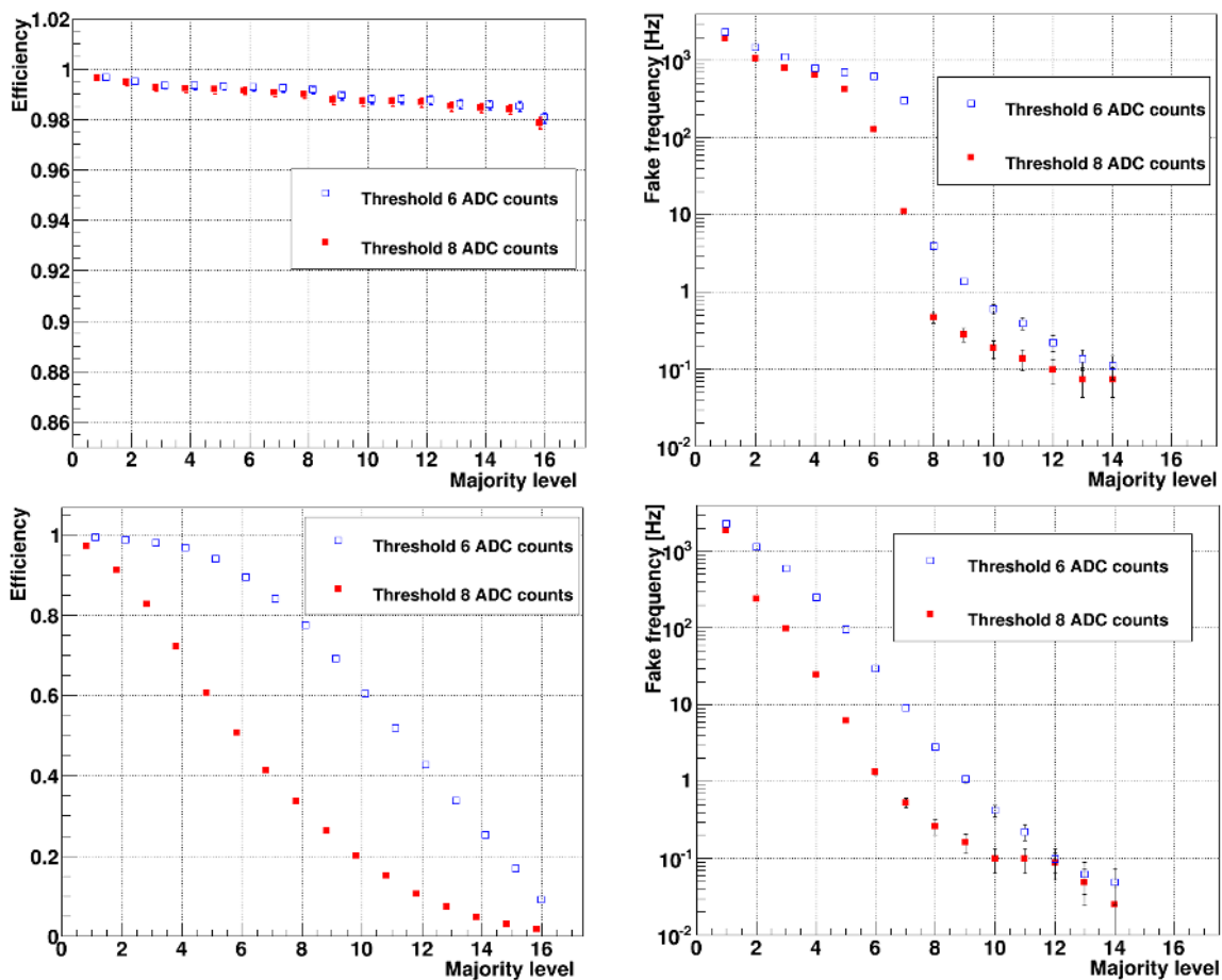
Figure 13. Top. Single GTO detection efficiency for vertical muon tracks (left) and corresponding rate of fake triggers (right) in Collection view as a function of the majority level for two different threshold values. The drop of the fake rate around MAJ = 7 is due to the exclusion of the noisy boards. Bottom. The corresponding GTO detection efficiency and fake rate as measured in Induction2 view. No fake triggers have been recorded for majority MAJ > 14 in both Collection and Induction2 views.
