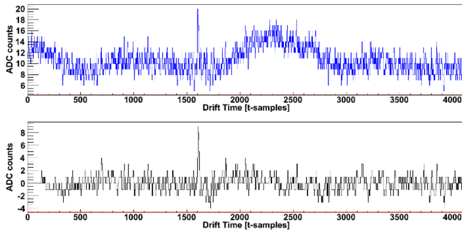
Figure 9. Top: typical waveform of a Collection wire signal, with both high and low frequency noise components. Bottom: waveform of the same signal after the application of the DR-slw algorithm.
