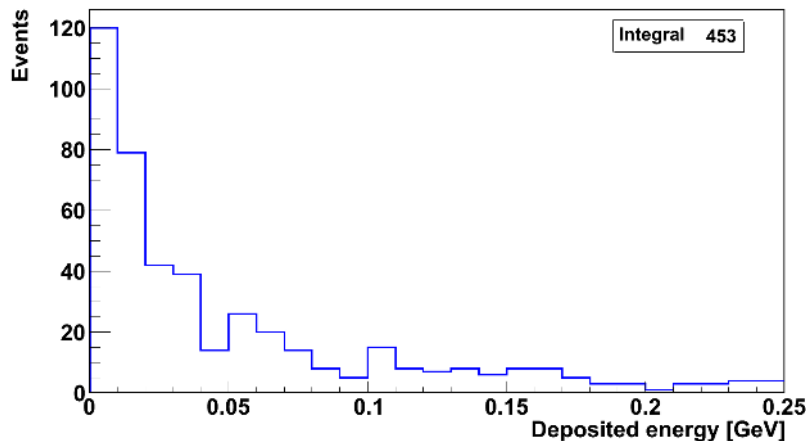
Figure 22. Distribution of the deposited energy of \nu NC MC interactions, not recognized by SD system with MAJ = 10 and GTO = 1, from a total of 10^4 generated events. Events below \sim 0.1 GeV are due to isolated converted gammas, neutrons and protons. The remaining is due to tracks projected over few Collection wires or shared between consecutive groups of 16 wires.
