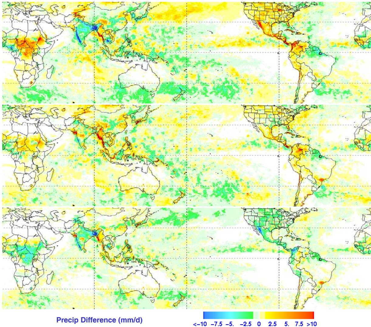
Fig. 3 Monthly average difference between (top) uncalibrated RT and V6, and (middle) calibrated RT and V6. (bottom) Improvement metric defined in Eq. 1, I_{cal} , which is the absolute value of the top image subtracted from the absolute value of the middle image. In all three panels the units are mm/d, the data are for July 2007, and the fields referenced are displayed in Fig. 2.
