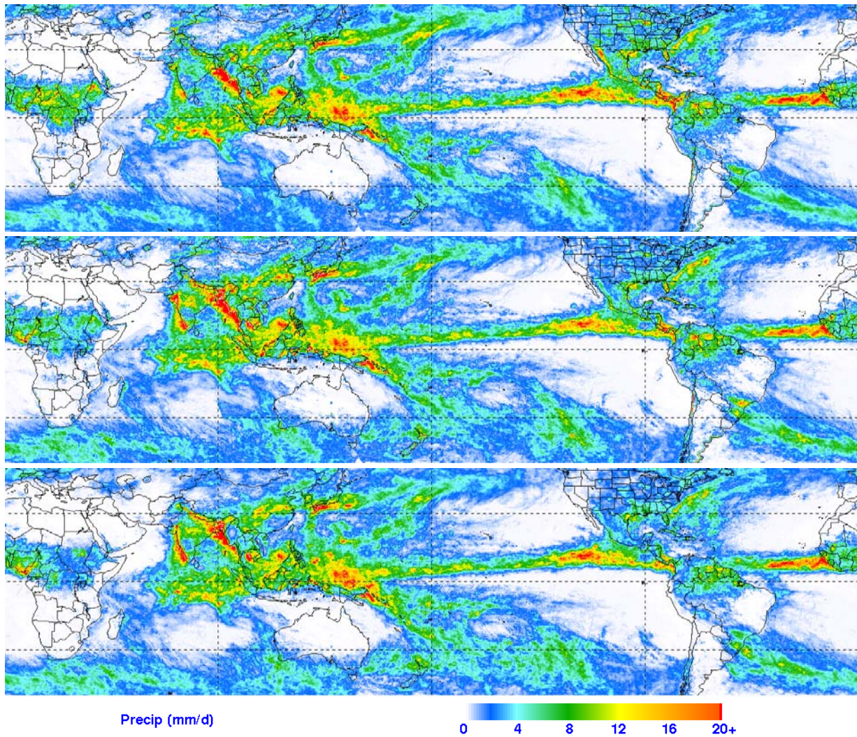
Fig. 2 Average precipitation rate in mm/d for July 2007 for the (top) uncalibrated RT, (middle) calibrated RT, and (bottom) V6 TMPA precipitation products.
