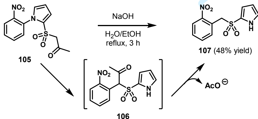
Scheme 33. Example of rearrangement of an N -arylated pyrrole yielding an N -unsubstituted pyrrole 101
