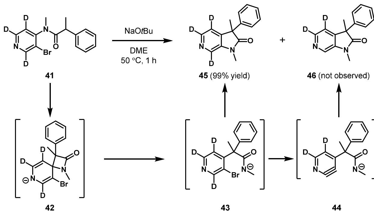
Scheme 15. Tandem Truce-Smiles rearrangement experiment to support S_NAr mechanism 52
