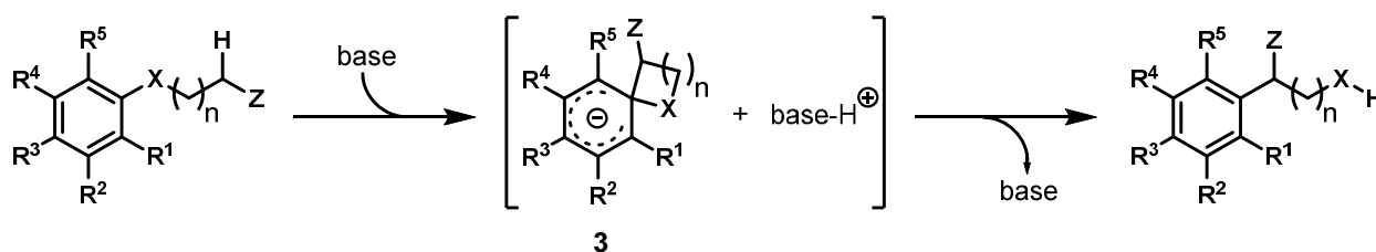
Scheme 3. General scheme of a base-catalyzed Truce-Smiles rearrangement
