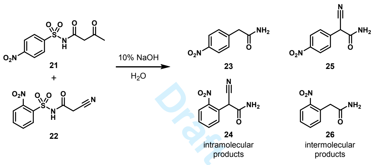
Scheme 9. Experiment demonstrating intramolecular mechanism 10
