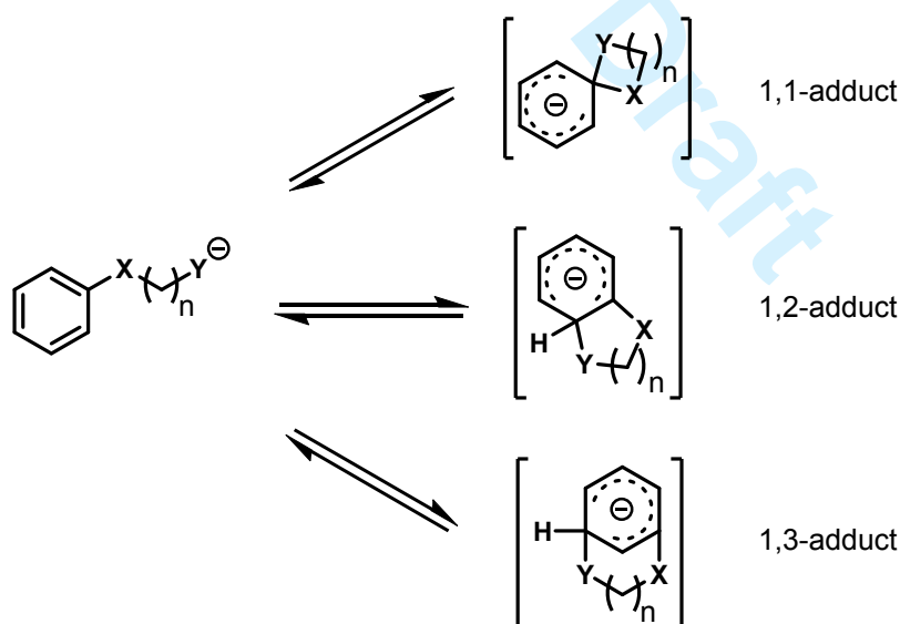
Figure 1. Isomers arising from addition of nucleophile during intramolecular nucleophilic aromatic substitution
