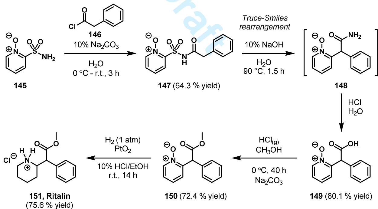
Scheme 40. Synthesis of Ritalin using Truce-Smiles rearrangement 12
