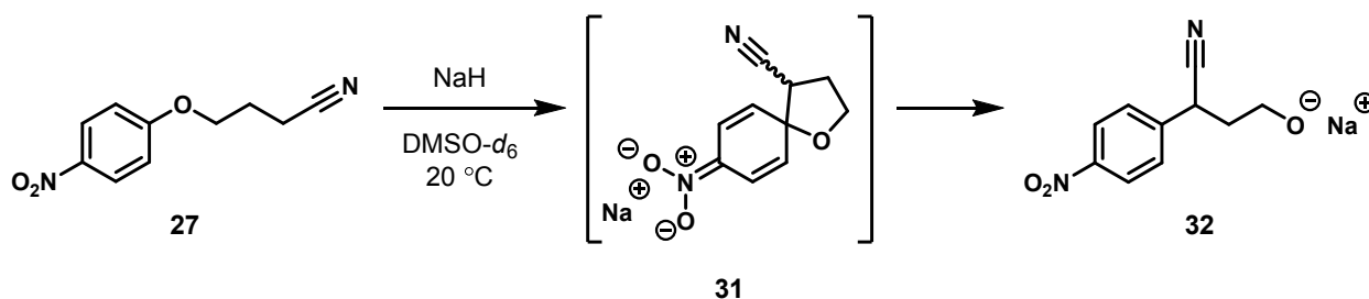
Scheme 11. Truce-Smiles rearrangement studied by 1 H and 13 C NMR spectroscopy 49
