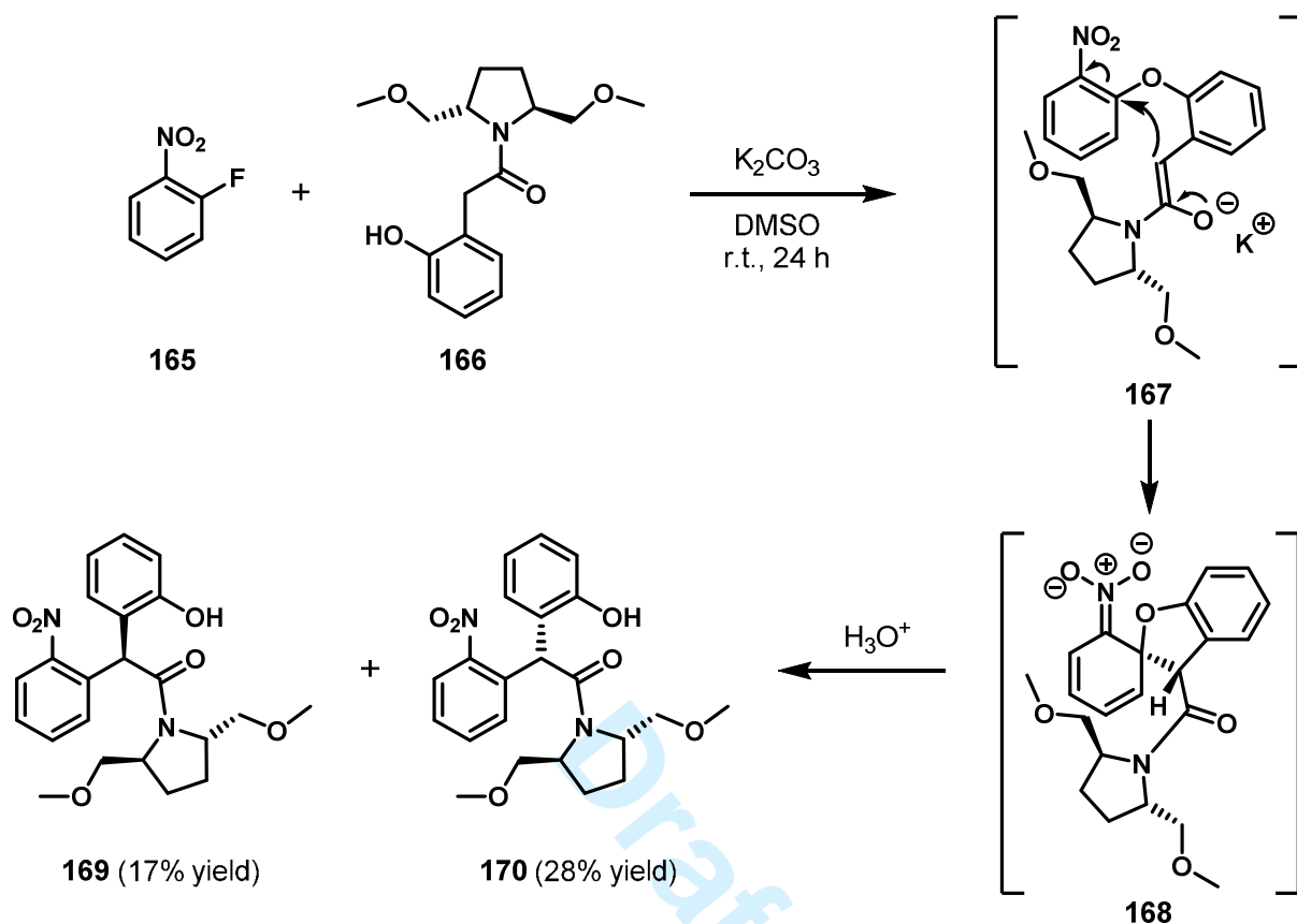
Scheme 44. Diastereoselective Truce-Smiles rearrangement 31
