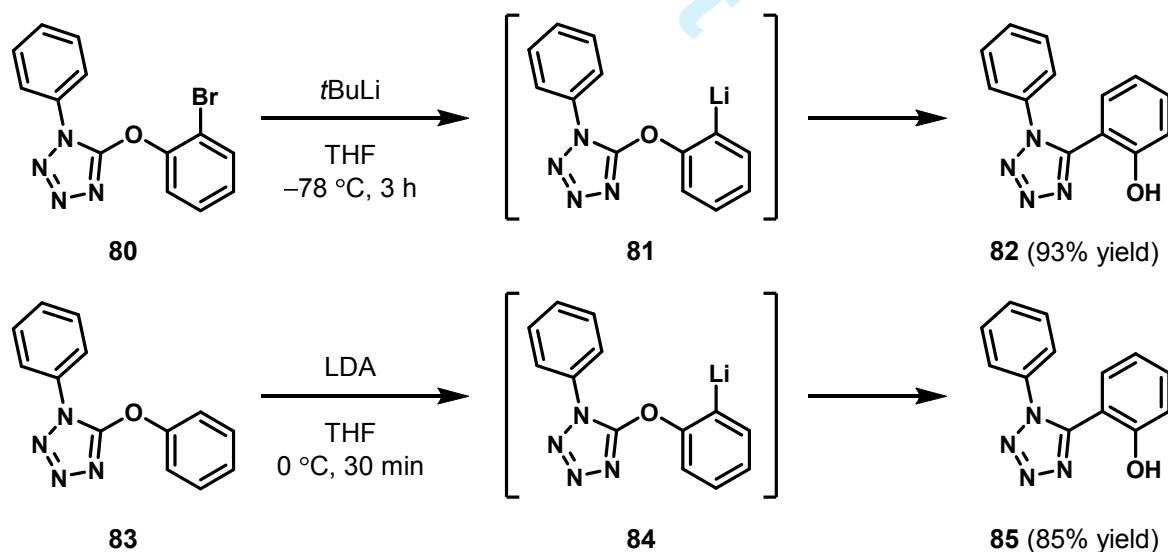
Scheme 28. Examples of successful rearrangement of tetrazole substrates 96
