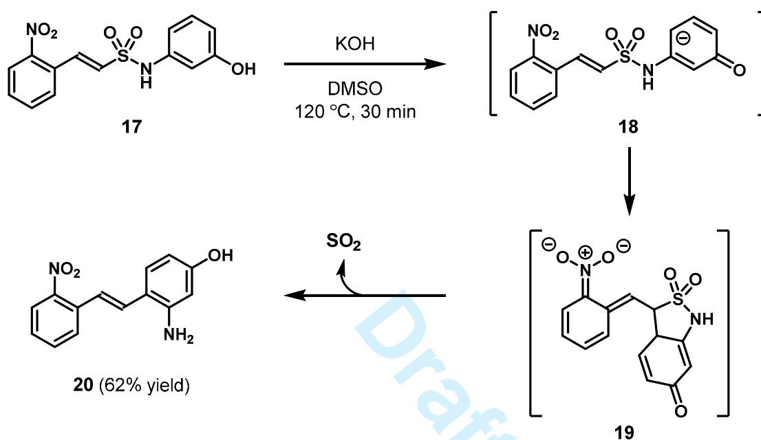
Scheme 8. Example of vinylogous Truce-Smiles rearrangement 35
