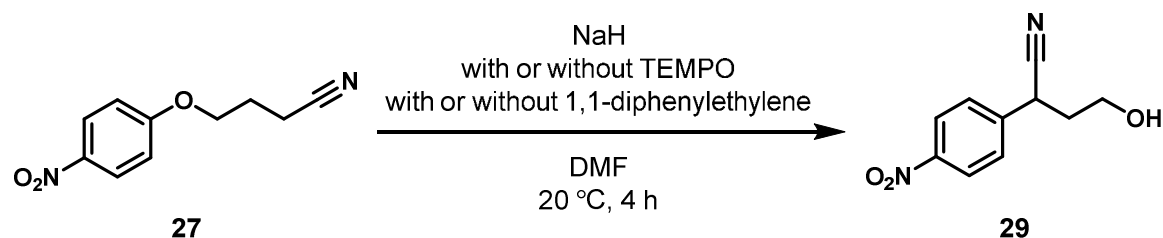
Scheme 17. Experiment probing existence of radical intermediates in Truce-Smiles rearrangement 49
