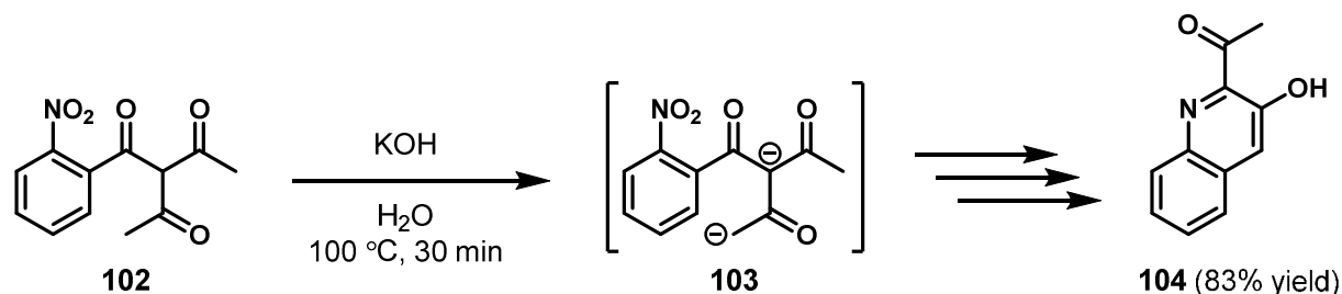
Scheme 32. Example of rearrangement of an aryl ketone and tandem cyclization yielding a quinoline 99
