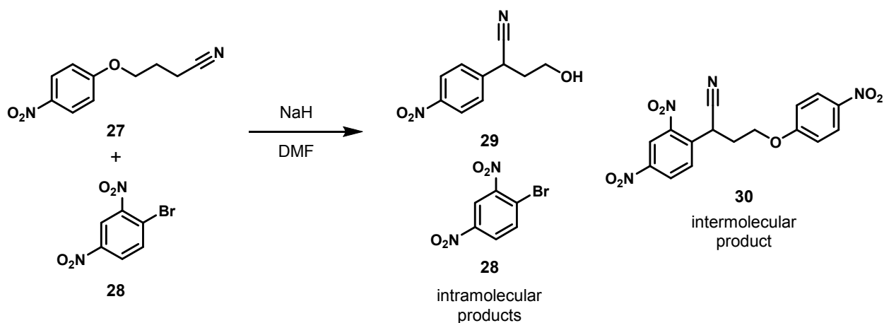
Scheme 10. Experiment demonstrating intramolecular mechanism 49
