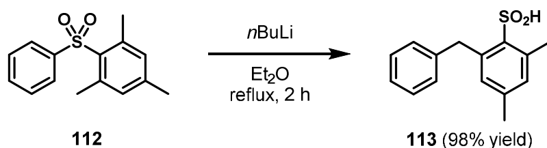
Scheme 36. Example of rearrangement of a diarylsulfone yielding a sulfinic acid 1
