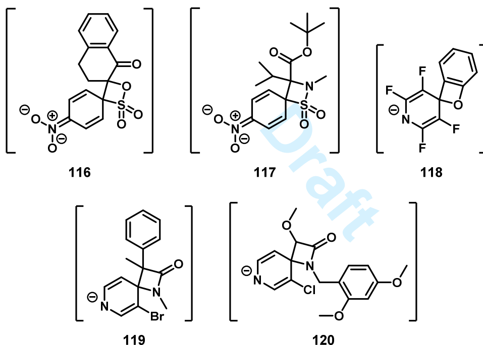
Figure 7: Putative reported 4-membered ring spirocyclic Meisenheimer adducts 36, 39, 48, 52, 95
