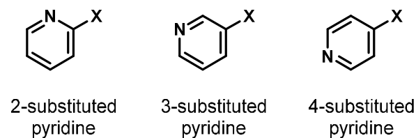
Figure 5. Substituted pyridine nomenclature
