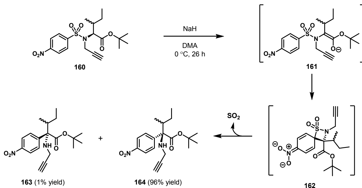
Scheme 43. Diastereoselective Truce-Smiles rearrangement 40
