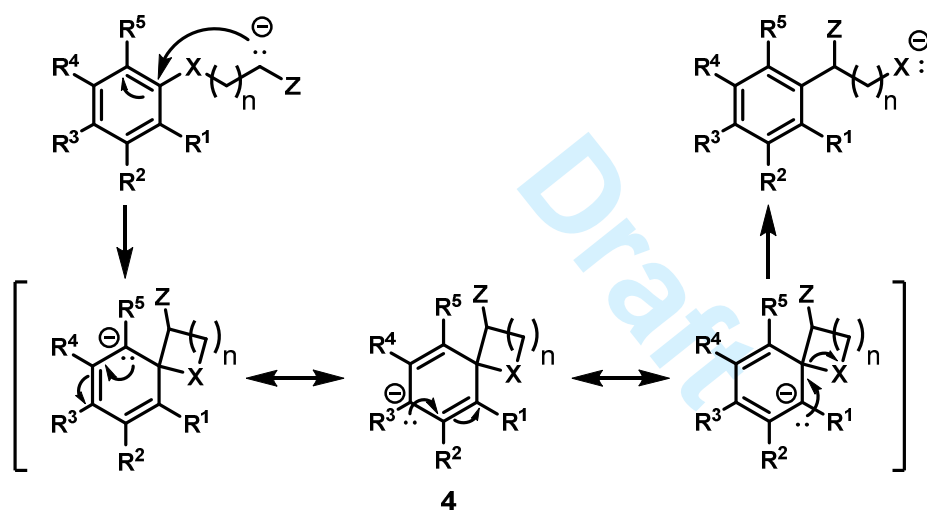
Scheme 4. Proposed S_NAr mechanism of the Truce-Smiles rearrangement
