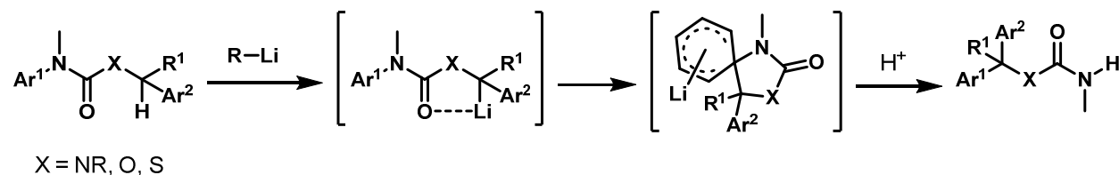
Scheme 19. General scheme for the Clayden rearrangement
