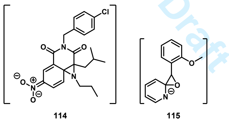
Figure 6: Putative reported 3-membered ring spirocyclic Meisenheimer adducts 47, 61
