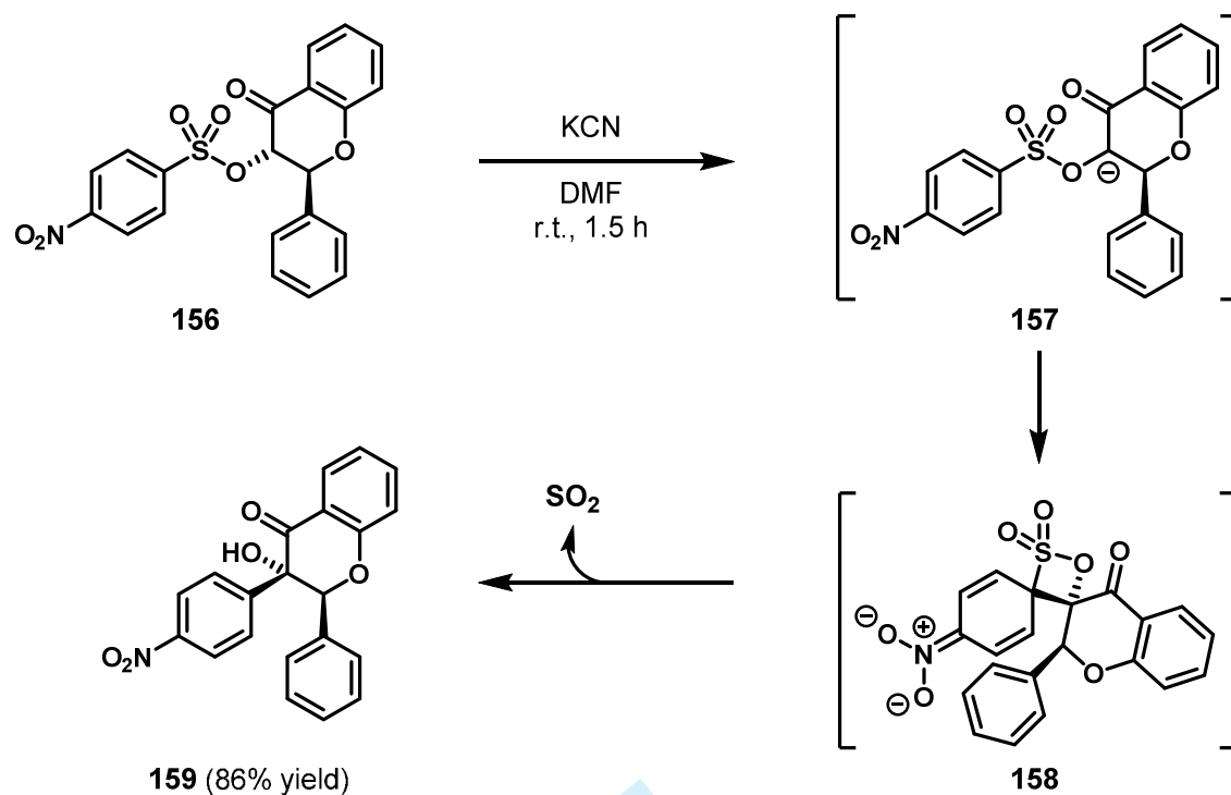
Scheme 42. Diastereoselective Truce-Smiles rearrangement 37
