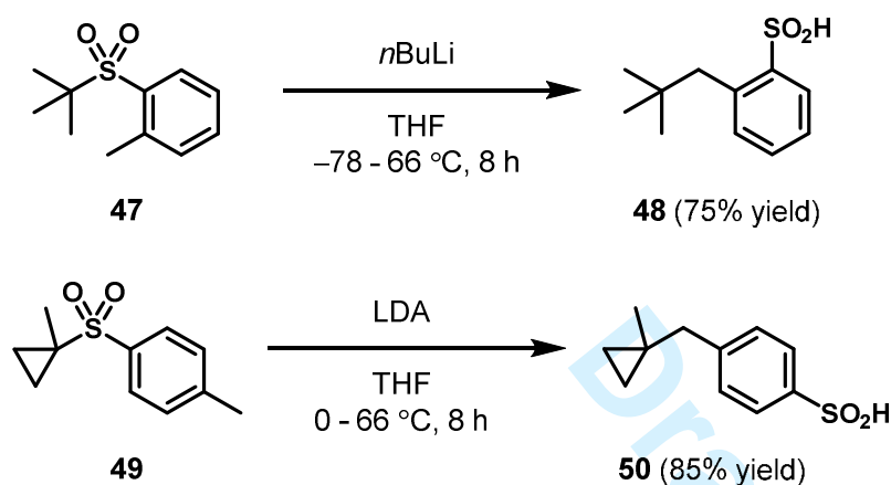
Scheme 16. Radical rearrangement reactions studied by Truce 7, 53
