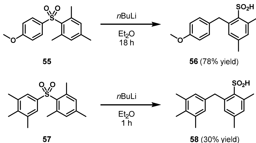
Scheme 22. Example of substrates bearing deactivating functional groups on the migrating ring 4
