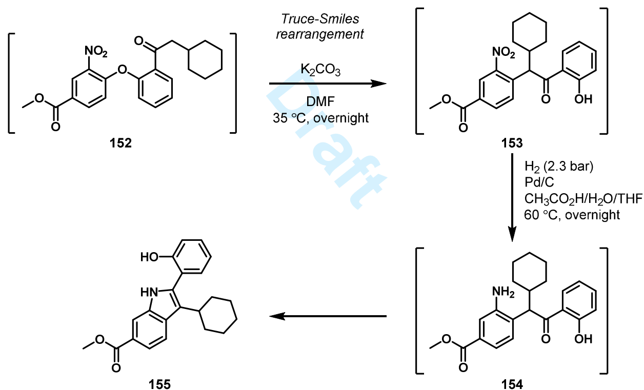
Scheme 41. Large-scale synthetic process involving Truce-Smiles rearrangement 45
