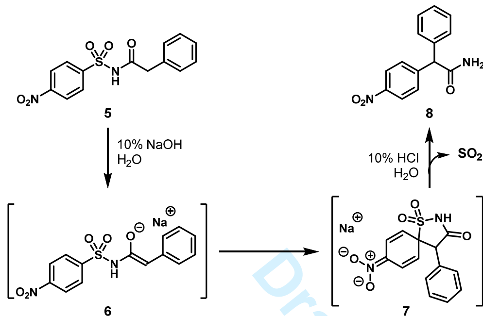
Scheme 5. Typical tandem Truce-Smiles rearrangement – sulfur dioxide extrusion reaction studied by Dohmori 9
