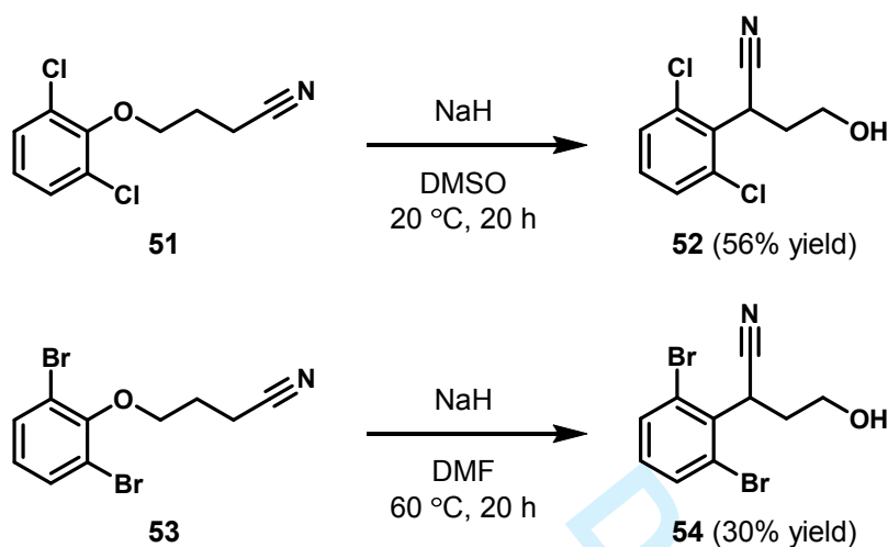
Scheme 21. Experiments demonstrating successful rearrangement of substrates bearing inductively-withdrawing substituents 49
