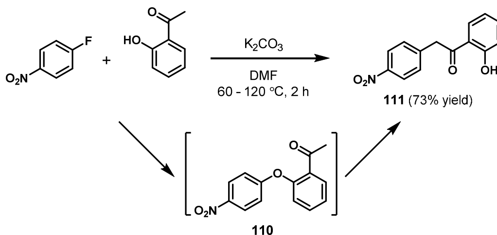
Scheme 35. Example of rearrangement of a diaryl ether yielding a phenol 44
