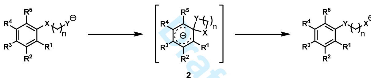
Scheme 2. General scheme of a Smiles rearrangement
