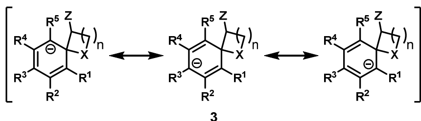
Figure 3. Resonance contributors to Truce-Smiles rearrangement Meisenheimer adduct
