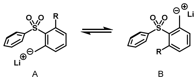
Figure 4. Conformational isomerism for ortho-substituted diarylsulfone substrates 3
