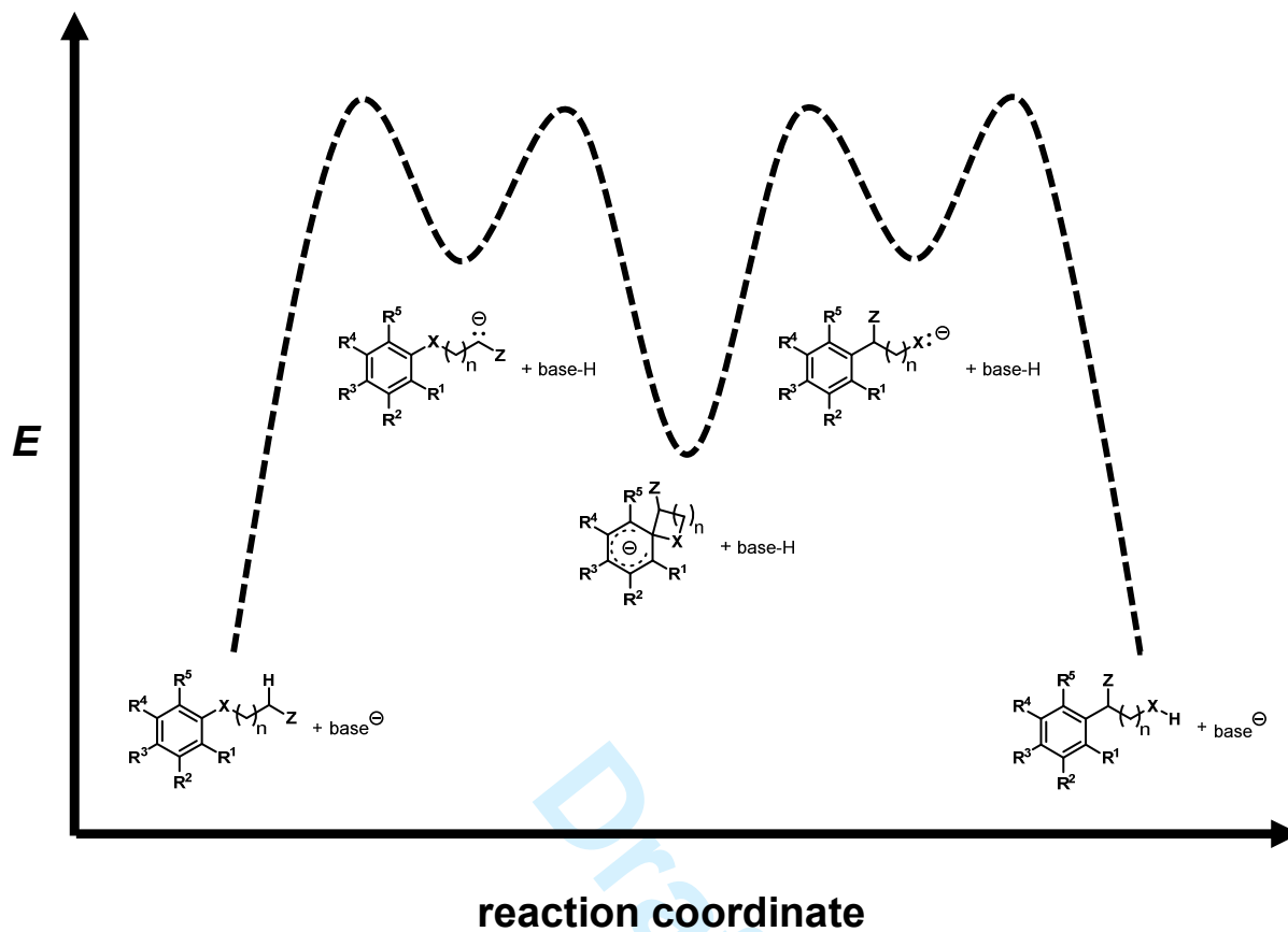
Figure 2. Expected energy diagram for typical Truce-Smith rearrangement assuming S_NAr mechanism
