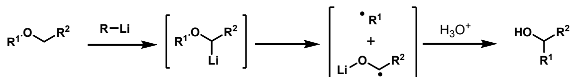
Scheme 18. General scheme for the [1,2]-Wittig rearrangement
