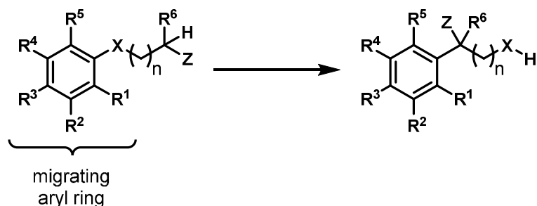
Scheme 20. Structural design variables of a Truce-Smiles rearrangement substrate
