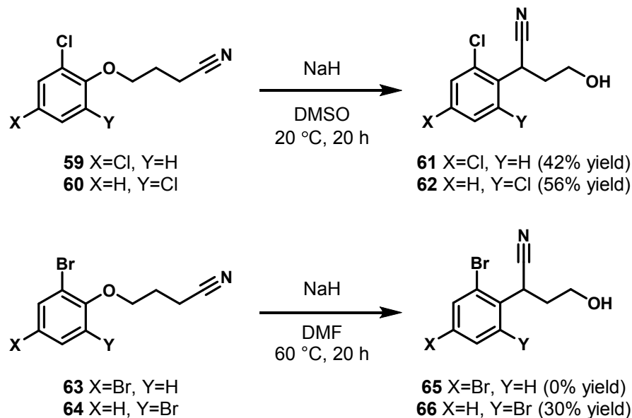
Scheme 23. Apparent ortho-substituent effect for migrating aryl ring 49
