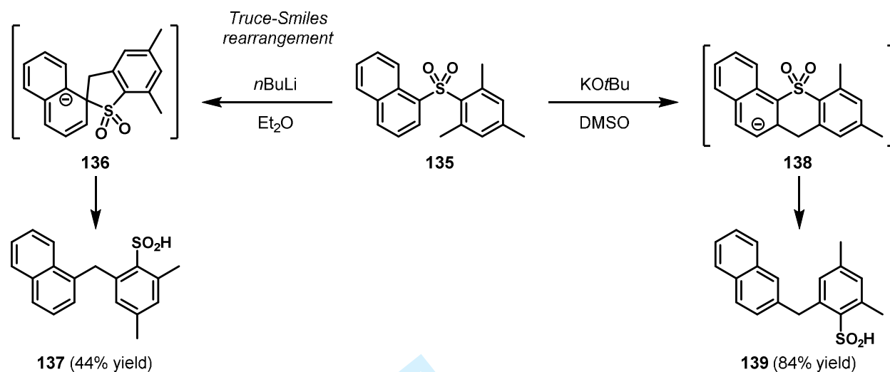
Scheme 38. Example of regioselective nucleophilic aromatic substitution reactions studied by Truce 6, 115
