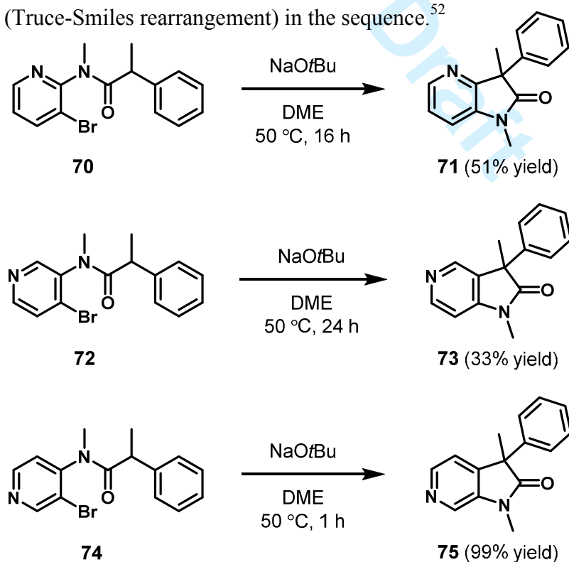
Scheme 25. Example of successful rearrangement of 3-substituted pyridyl substrate and comparison to 2- and 4-substituted analogs 52
