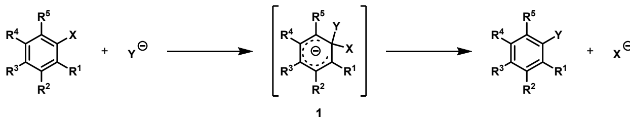
Scheme 1. General scheme for S_NAr mechanism
