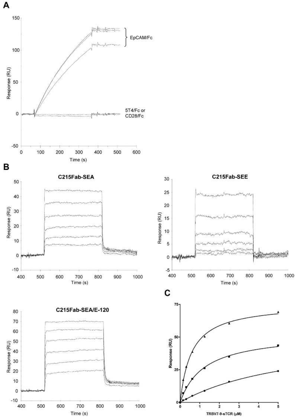
Figure 6. Surface plasmon resonance analysis of TRBV7-9 binding to fusion proteins containing SEA, SEE and SEA/E-120. A) Sensorgrams obtained after injection (5 min at 20 \mu\text{L}/\text{min} ) of 25 nM C215Fab-SEA, -SEE and -SEA/E-120 over amine coupled EpCAM/Fc (density \sim 870 RU). Capture levels of 109, 134 and 133 were calculated for C215Fab-SEA, -SEE and -SEA/E-120 respectively. No binding was observed when these samples were injected over CD28/Fc (density \sim 680 RU) or 5T4Fc (density \sim 990 RU). B) Sensorgrams showing binding of 0.156 to 5 \mu\text{M} TRBV7-9 to EpCAM captured C215Fab-SEA, C215-SEE or C215-SEA/E-120 after subtraction of sensorgram with sample buffer. C) Response levels at t \sim 530 s plotted against TRBV7-9 concentration for binding to SEA (squares), SEE (circles) and SEA/E-120 (triangles) fusion proteins. Curves were fit to a one-site hyperbola model in GraphPad Prism for calculation of maximal response and apparent affinity.
