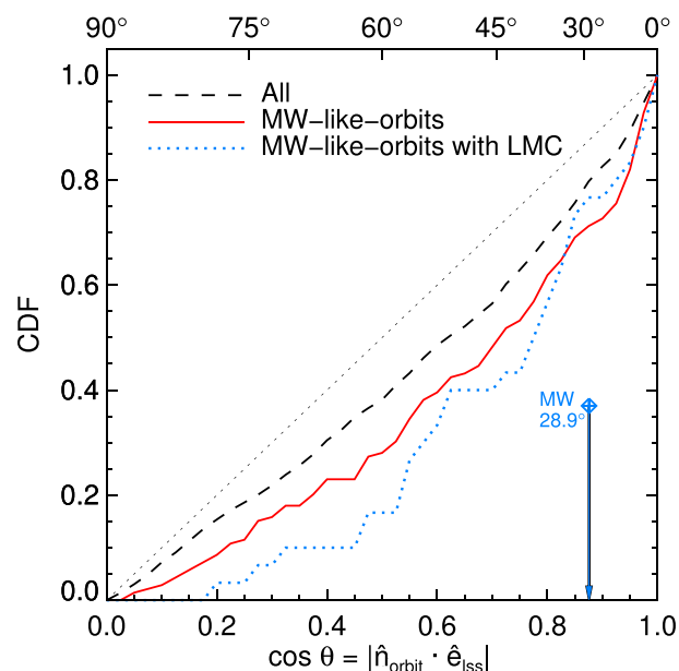
Figure 5. The CDF of the alignment angle, \cos \theta , between the common orbital pole of satellites and, the normal, \hat{e}_{\text{LSS}} , to the large-scale sheet in which the system is embedded. We show results for three samples: the full population of MW mass systems (dashed black), the MW-like-orbit systems (solid red), and the MW-like-orbit systems that also have an LMC mass satellite (dotted blue). The arrow indicates the measurement for our galaxy, which we obtained using the LSS directions provided by Libeskind et al. (2015).
