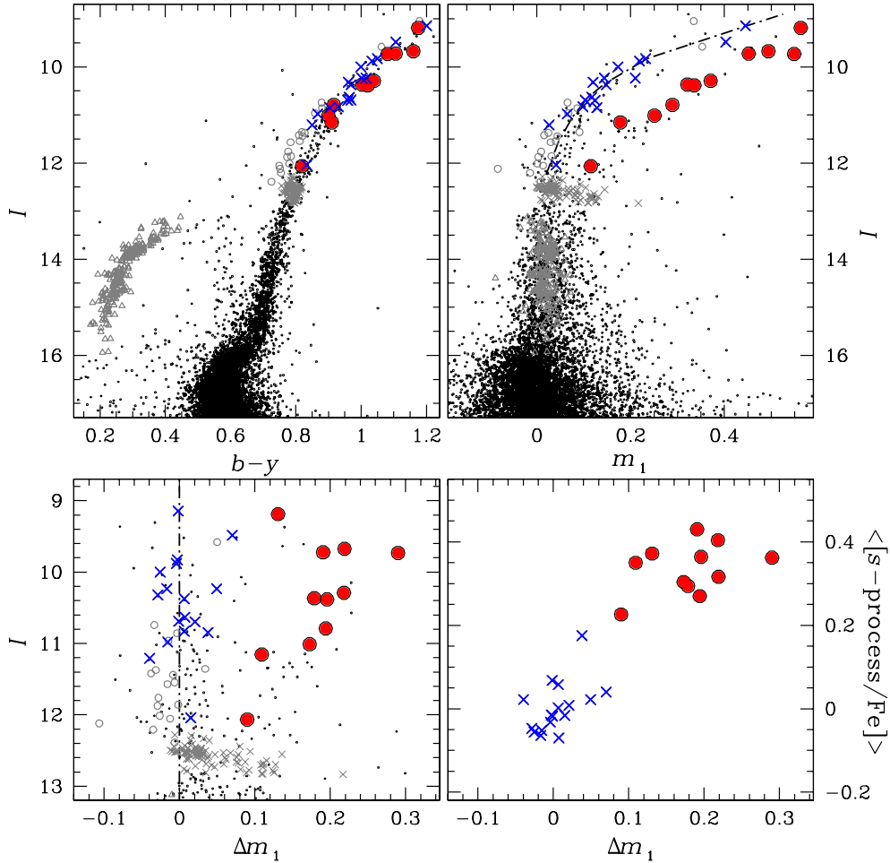
Fig. 19. Top panels: I-b-y (left) and I-m_1 (right) CMD for M22, corrected for differential reddening. The grey symbols represent HB stars (triangles), probable AGB stars (circles) and RGB bump stars (crosses) selected in the I-(b-y) CMD. Spectroscopic data are superimposed with s -rich stars represented by red circles, and s -poor stars by blue crosses, according with the other figures. Bottom panels: colour difference \Delta m_1 between each analyzed star and a reference fiducial line represented as a dotted line (left panel). On the right panel the \langle [s/\text{Fe}] \rangle average abundances are shown as a function of \Delta m_1 . The sources for the photometric data are given in Sect. 2.
