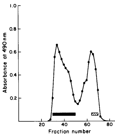
FIG. 2. Purification of S. suis type 2 polysaccharide on Sepharose 6B column ( 2.5 \times 180 cm) in M/30 PO_4 buffer pH 8.0. Polysaccharides were analyzed by phenol-sulfuric acid assay. Solid and hatched bars indicate the capillary precipitin test against type 2 and teichoic acid antisera, respectively.
