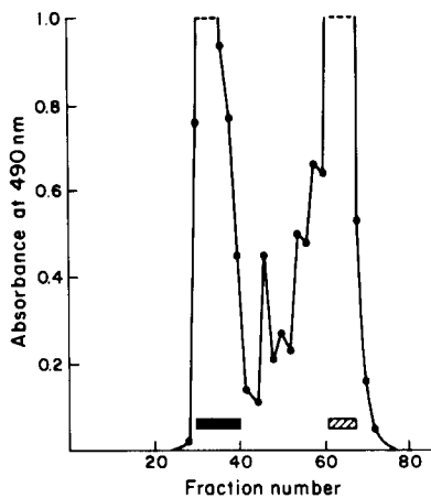
FIG. 1. Purification of S. suis type 1 polysaccharide on Sepharose 6B column ( 2.5 \times 180 cm) in M/30 PO_4 buffer pH 8.0. Polysaccharides were analyzed by phenol-sulfuric acid assay. Solid and hatched bars indicate the capillary precipitin test against type 1 and teichoic acid antisera, respectively.
