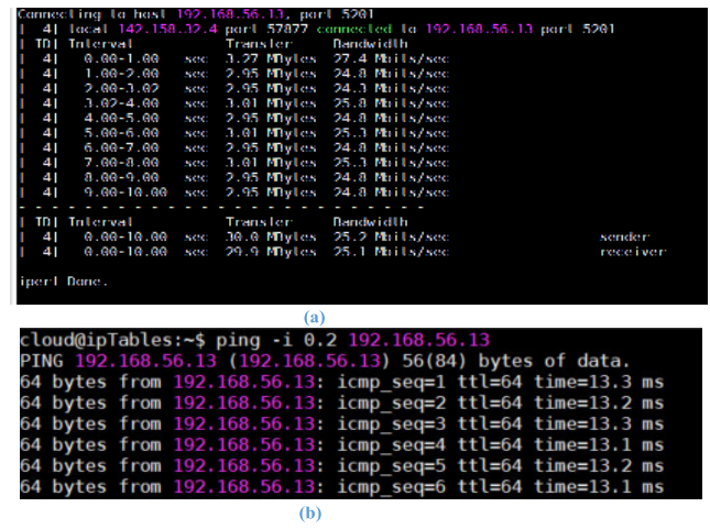
FIGURE 14. (a) iperf data rate received on the LiFi-xc dongle at the UoB (b) IP ping e2e delay (latency) UoE-UoB.
