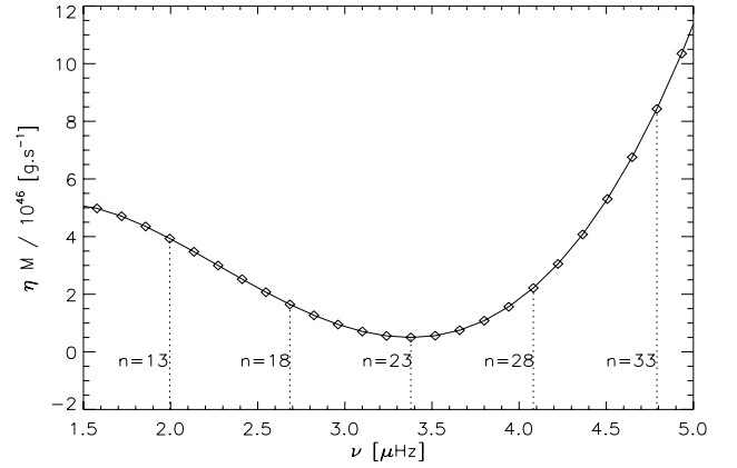
Fig. A.1. Product of the damping rates ( \eta ) multiplied by the mode mass ( M ) versus mode frequency. The vertical dotted lines identify radial mode orders.
