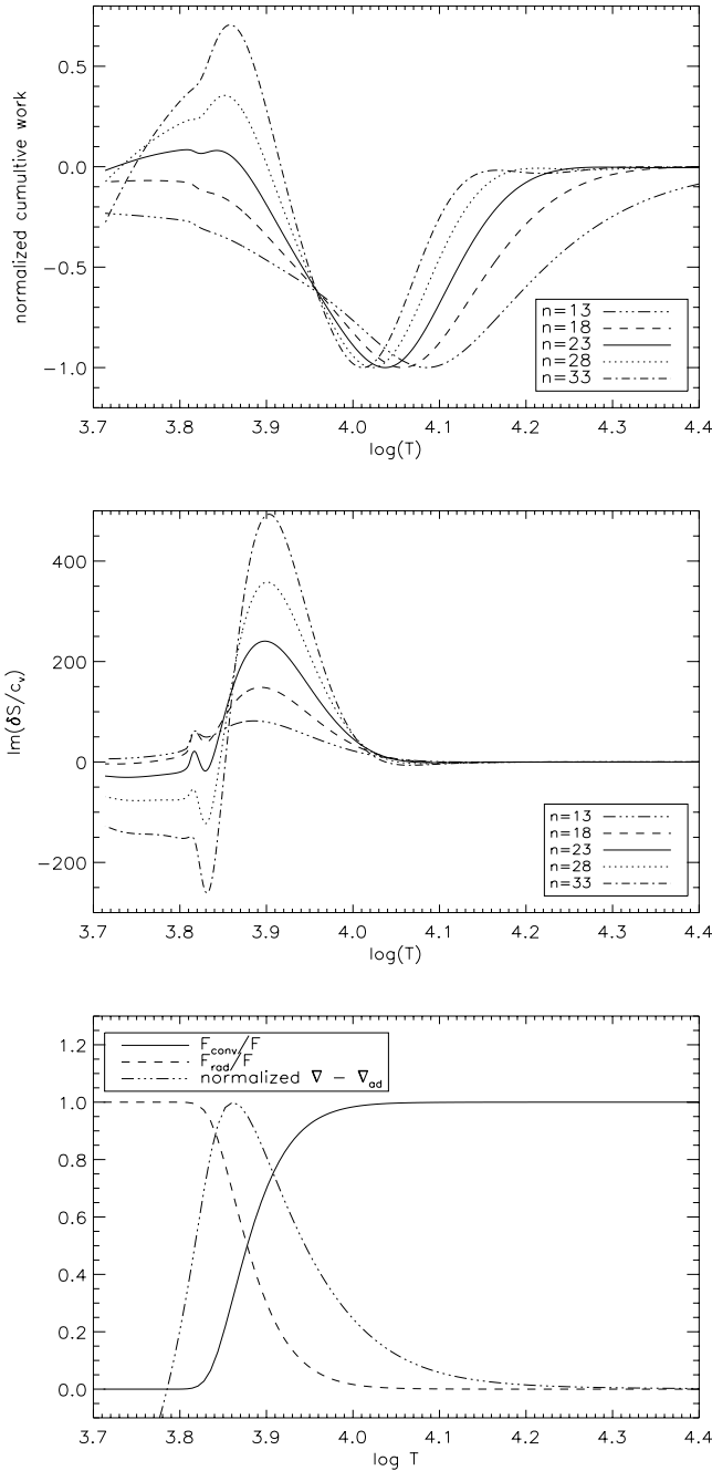
Fig. A.2. Top: normalized cumulated work integral versus logarithm of temperature for five values of eigenfrequencies. These modes are emphasized in Fig. A.1. Middle: imaginary part of the Lagrangian perturbation of entropy versus logarithm of temperature. Bottom: normalized convective and radiative fluxes versus logarithm of temperature. The difference between the real and adiabatic gradient ( \nabla ) is also plotted and normalized to its maximum.
