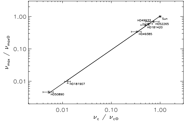
Fig. 1. Frequency of the maximum of oscillation power for the main-sequence and red-giant stars of Table 1 as a function of the frequency cut-off. All quantities are normalized to the solar values.
