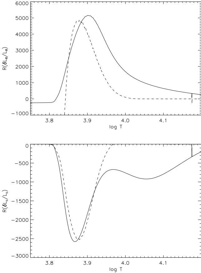
Fig. A.3. Top: real part of the radiative luminosity perturbation for the mode of radial order n = 23 versus logarithm of temperature. The solid line represents the full non-adiabatic computation as described in Sect. A.1, while the dashed line represents the approximate expression given by Eq. (A.6). The rapid variation near \log T = 4.17 is the result of the presence of a node of the eigenfunction. Bottom: real part of the convective luminosity perturbation for the mode of radial order n = 23 versus logarithm of temperature. The solid line represents the full non-adiabatic computation as described in Sect. A.1, while the dashed line represents the approximate expression given by Eq. (A.7).
