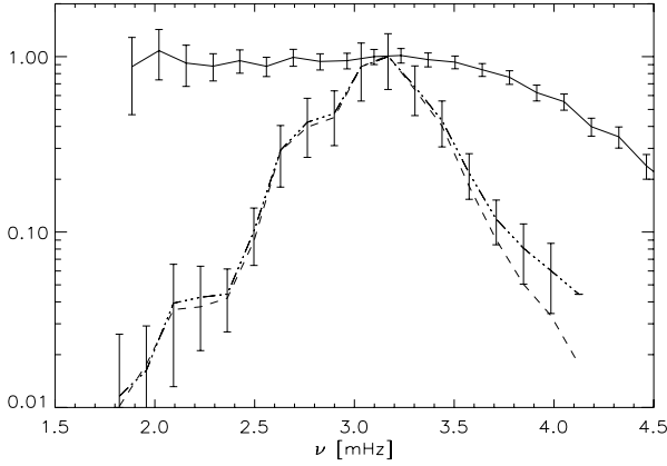
Fig. 2. Normalized 1/(2\Theta^2) (dashed-dots line), where \Theta = \eta M , and \Pi = \mathcal{P} M (solid line) computed from solar seismic data from the GOLF instrument (Baudin et al. 2005). The normalized mode height ( H ) corresponds to the dashed line. All quantities are normalized to unity at the frequency of \nu = \nu_{\max} . The associated mode masses are computed as described in Belkacem et al. (2006).
