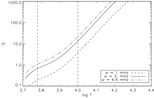
Fig. 3. Product Q (see Eq. (9)) versus the logarithm of the temperature for three values of the mode frequency for a solar model described in Appendix A. Vertical dotted lines delimit the limits of super-adiabatic gradient (see Fig. A.2 bottom panel).
