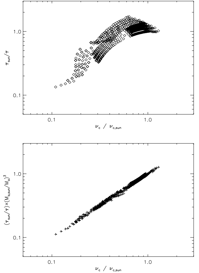
Fig. 4. Top: thermal frequency ( 1/\tau ) computed from Eq. (9) versus the cut-off frequency computed following Eq. (1), normalized to the solar values, for models with masses ranging from M = 1 M_{\odot} to M = 1.4 M_{\odot} (with an increment of 0.05 M_{\odot} ) and from the ZAMS to the ascending vertical branch. Bottom: the same as for the top panel, except the thermal frequency is divided by the Mach number to the third versus the normalized cut-off frequency.
