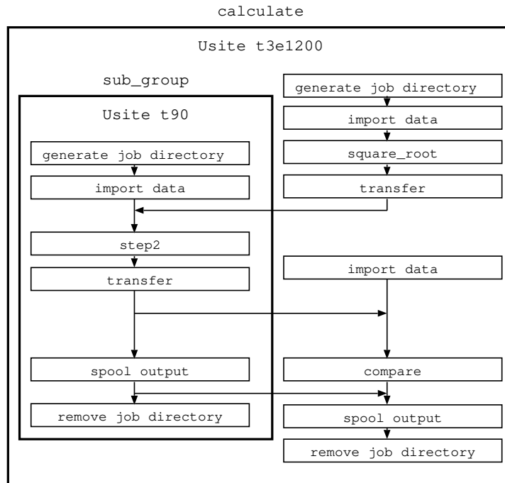
Fig. 4. AJO for job example.
