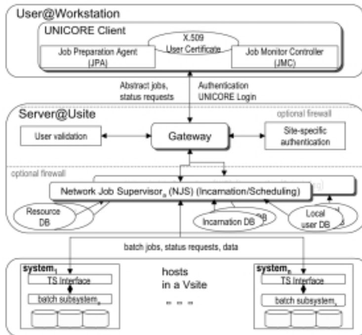
Fig. 2. Detailed architecture.
