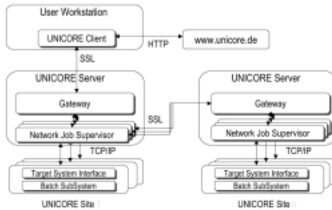
Fig. 1. Architecture overview.
