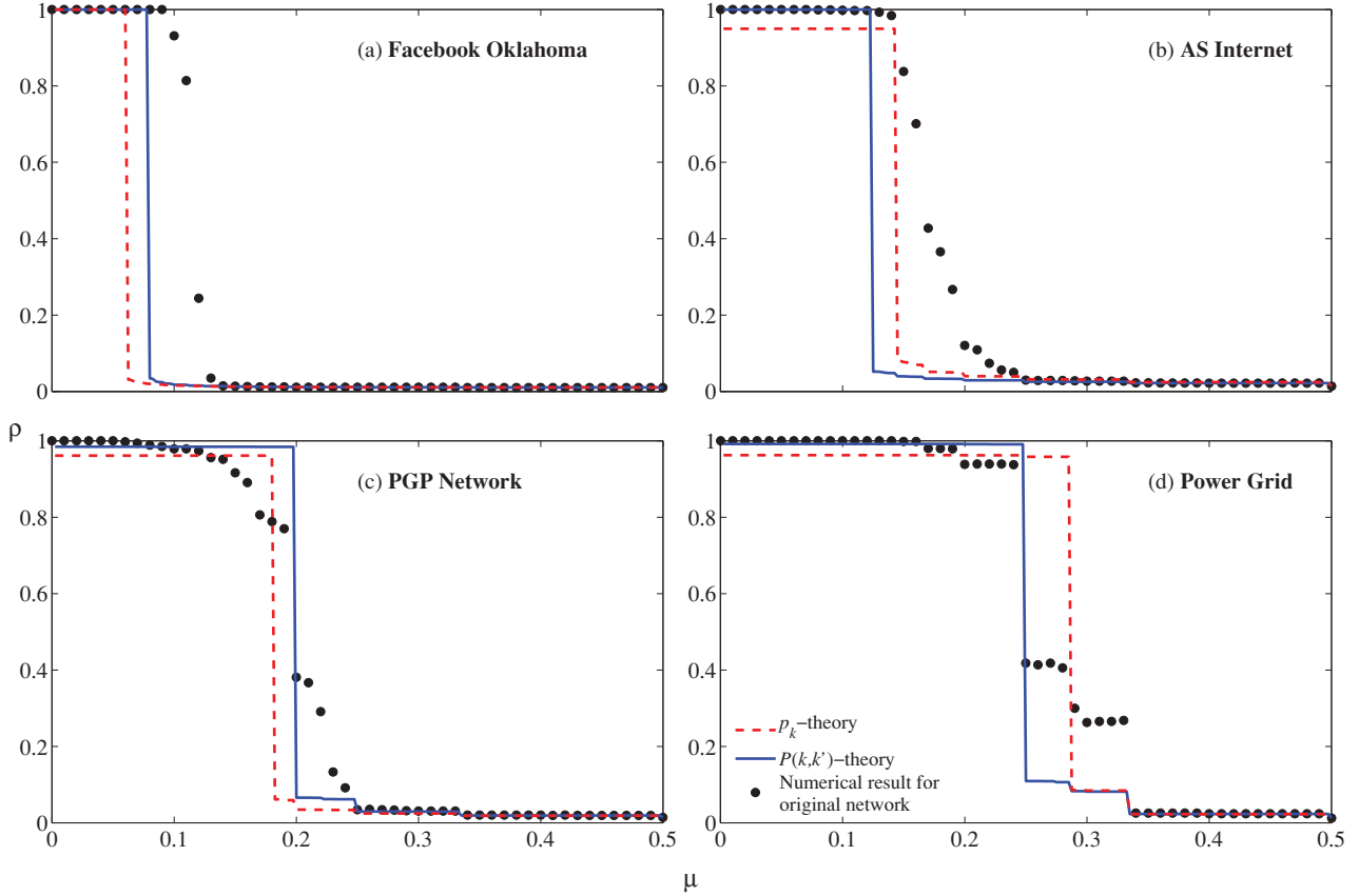
FIG. 7. (Color online) Watts threshold model, with threshold mean \mu and variance \sigma^2 = 0 (that is, with uniform thresholds) for the networks from Fig. 1. We use a seed fraction of \rho_0 = 10^{-2} .
