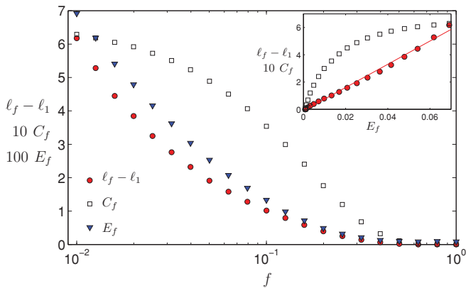
FIG. 5. (Color online) Watts-Strogatz small-world network: We plot \ell_f - \ell_1 (red circles), 10 C_f (open squares), and 100 E_f (blue triangles) as functions of rewiring fraction f . (See the main text for the definitions of these quantities.) The inset shows \ell_f - \ell_1 and C_f as functions of E_f for f \geq 10^{-2} . Observe the linear relation between E_f and \ell_f - \ell_1 , which suggests that \ell_f - \ell_1 might be a good indicator of how well the bond-percolation process on a network can be approximated by tree-based theory.
