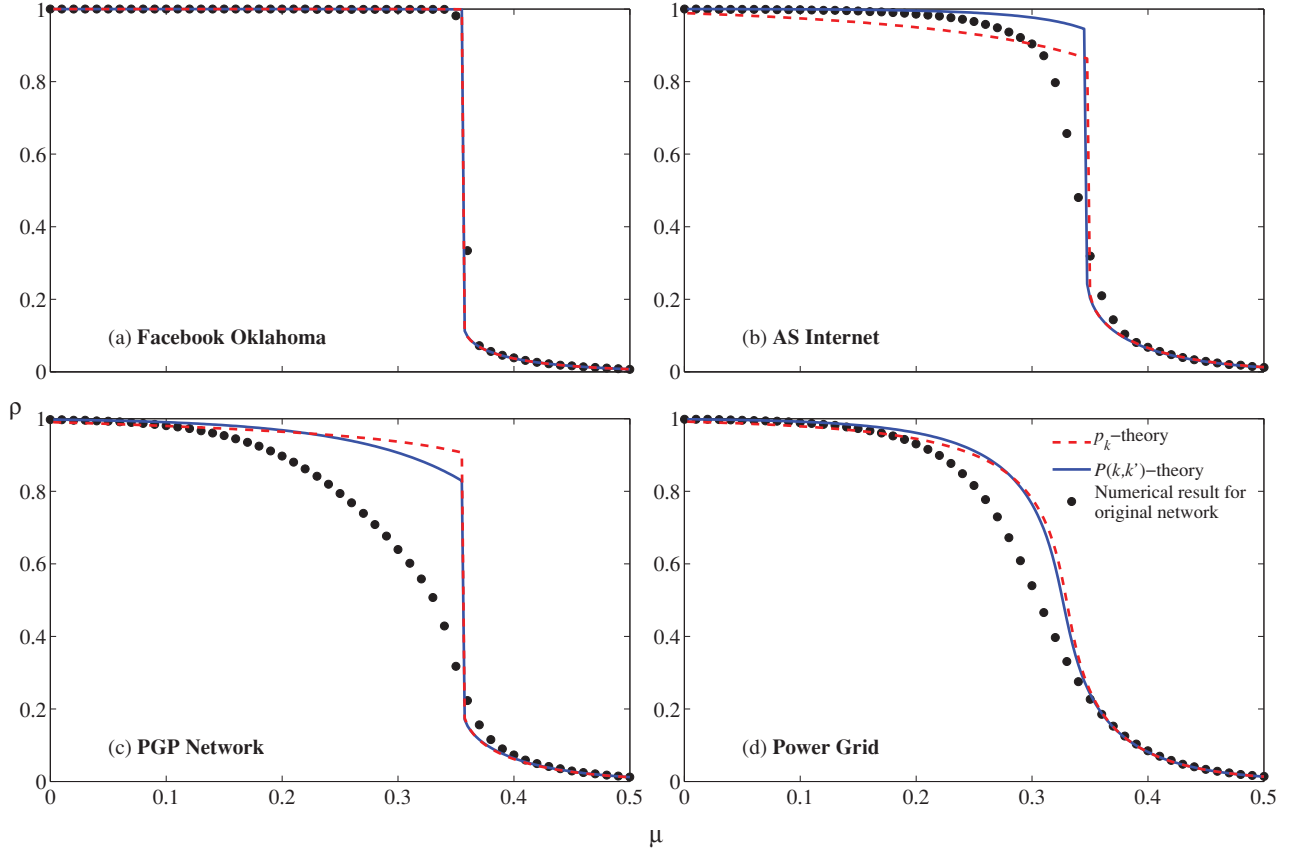
FIG. 3. (Color online) Watts threshold model, with threshold mean \mu and variance \sigma^2 = 0.04 , for the networks from Fig. 1. We use the seed fraction \rho_0 = 0 because the nodes with negative thresholds immediately turn on and act as seeds. In other words, the effective seed fraction is given by the value of the cumulative distribution function of the thresholds evaluated at zero. This fraction is [1 + \text{erf}\{-\mu/(\sigma\sqrt{2})\}]/2 .
