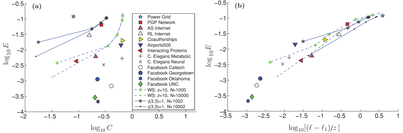
FIG. 6. (Color online) Scatter plots of \log_{10} E versus (a) \log_{10} C (with R^2 \approx 0.087 ) and (b) \log_{10}[(\ell - \ell_1)/z] (with R^2 \approx 0.94 ).
