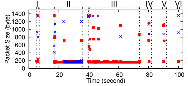
Fig. 4. The IPSec packets of six Wi-Fi calling events over time (×: uplink packets; ■: downlink packets; I/VI: Activating/Deactivating Wi-Fi calling; II/III: Receiving/Dialing a call; IV/V: Sending/Receiving a text).
