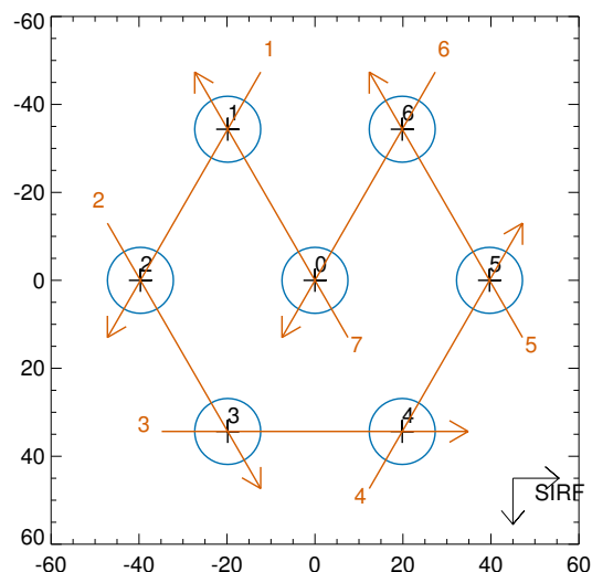
Fig. 7. Example of the pattern of the scans in the array-pointing mode. The unit of the x - and y - axes is in arcsec, and the direction of the axis follows the science instrument reference frame (SIRF), which is the coordinate system that we use for the pointing measurements. The black crosses with blue circles indicate the pixels with their HPBW of 15'' , and the red arrows indicate the scan direction.
