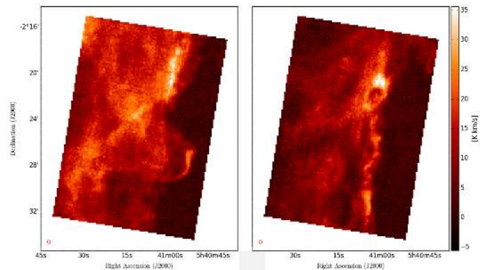
Fig. 11. Example of large scale mapping of the Horsehead nebula region, performed in four hours, covering a 17.5' \times 12.5' field. The lower left red circle show the 15'' beam. We display two integrated channel maps at 9.5–11.3 \text{km s}^{-1} and 13–15 \text{km s}^{-1} , delineating the complex kinematics of the region. While strikingly prominent at optical wavelengths where it is seen as a dark patch, the Horsehead nebula [CII] emission is limited to the UV-illuminated edge of its PDR. The fine morphology of the IC 434 PDR interface displays beautifully.
