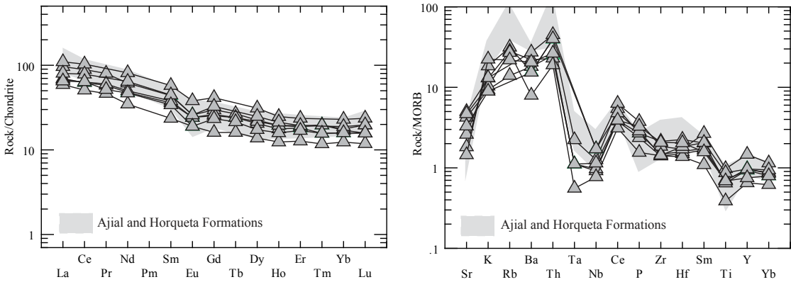
FIG. 7. Chondrite-normalized Rare Earth elements (REE) patterns and MORB-normalized trace elements patterns for volcanic rocks from the Río Damas Formation in the principal cordillera. Data from Ajjal and Horqueta Formations in the Coastal Cordillera of Central Chile are after Vergara et al. (1995). Normalizing values are from Sun and McDonough (1989) (Chondrite) and Pearce (1983) (MORB).
