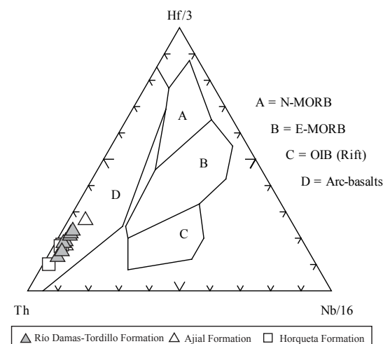
FIG. 10. Tectonic setting discrimination diagram (Cabanis and Lecolle, 1989) for volcanic (basic-intermediate) rocks in the studied area. Ajial and Horqueta Formation samples in the Coastal Cordillera in Central Chile after Vergara et al. , 1995.
