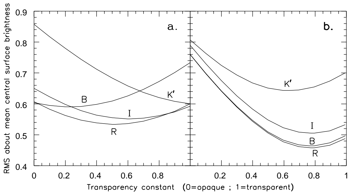
Figure 2: Dispersion about the mean central surface brightness as the transparency constant C is varied. Separate curves are given for the B , R , I , K' passbands. Panel a relates to the HSB sub-sample and panel b relates to the LSB sub-sample.
