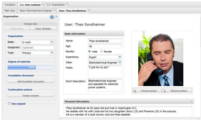
Fig. 7. Persona model in UsER (Image courtesy of stockimages / FreeDigitalPhotos.net)
