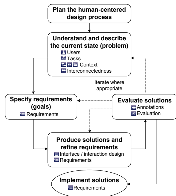
Fig. 1. The Basic Process Model for UsER
