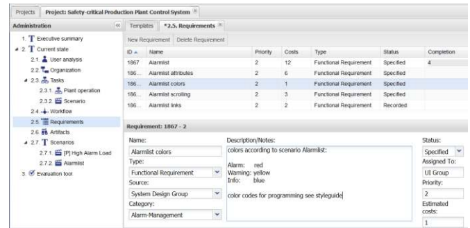
Fig. 10. Hierarchical requirements structures in UsER with IDs, descriptions, states, priorities and project-specific grouped categories
