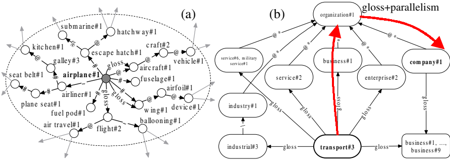
Fig. 5. a) example of semantic net for airplane#1 b) example of intersecting semantic patterns for transport#3 and company#1 .
