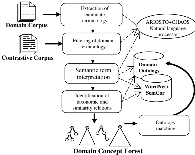
Fig. 3. Architecture of OntoLearn.
