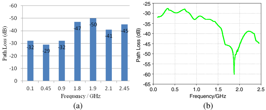
Figure 5. Path loss for the capsule position at A (upper esophagus): (a) with exact tissue property; (b) with the tissue property considered in Table 2.
