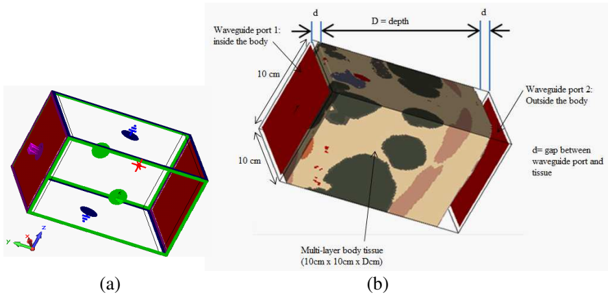
Figure 3. (a) Boundary condition; (b) simulation setup for investigating path loss in the body channel.
