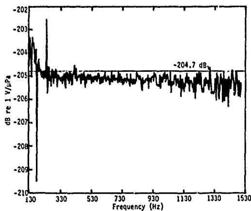
Fig. 22. F37 receiving response obtained by broadband methods with the F36 as the standard (one cycle of 1-kHz signal).
