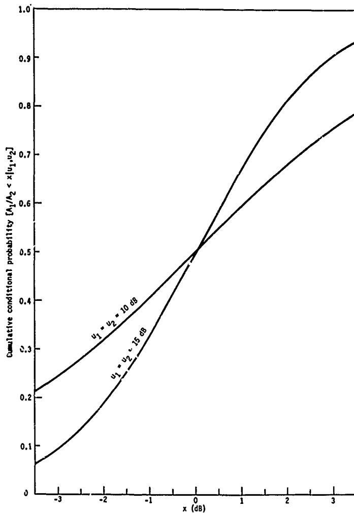
Fig. B4. Cumulative conditional probabilities of the quotient of two modified Rician variables; \sigma_1 = \sigma_2 = 0 dB.
