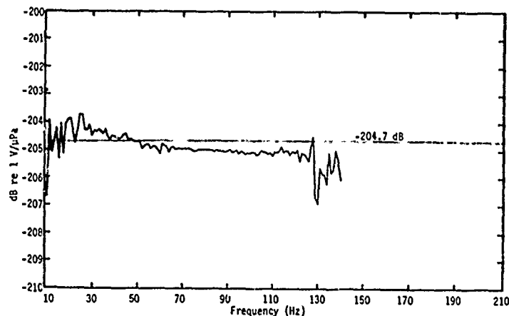
Fig. 15. F37 receiving response obtained by broadband methods with the F50 as the standard (one cycle of 65-Hz signal).
