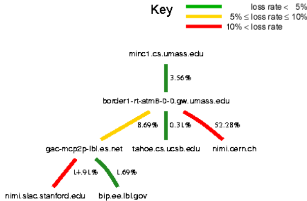
Figure 6: MINT view of the logical multicast tree with losses.
