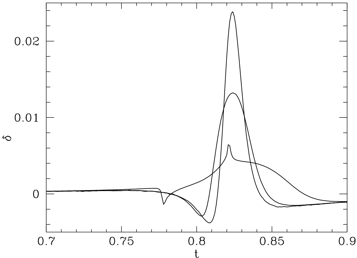
FIG. 5.—Comparison of planetary deviation light curve for different source radii: u_* = 0.003, 0.01, \text{ and } 0.03 , corresponding to R_* = 3 R_\odot with lens at 4 kpc, R_* = 10 R_\odot with lens at 4 kpc, and R_* = 10 R_\odot with lens at 7 kpc, respectively. The deviation \delta is plotted vs. the time in units of t_E . These curves are for q = 10^{-4} , x_p = 1.3 , u_{\min} = 0.02 , and \beta = 50^\circ . The smaller the stellar radius, the higher and sharper the deviation. The bumps in the u_* = 0.03 radius curve occur as the limb of the star crosses the central caustic.
