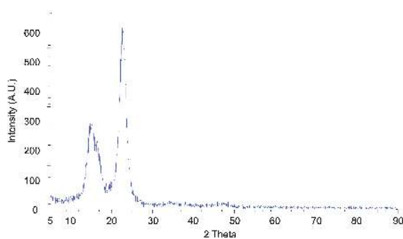
Figure 1 X-ray powder diffraction pattern of lyophilized nanocrystalline cellulose. Intense peaks at 15^\circ and 23^\circ 2\theta , due to constructive interference of diffracted x-rays, in addition to the lack of an amorphous halo, indicate the highly crystalline nature of the material.
