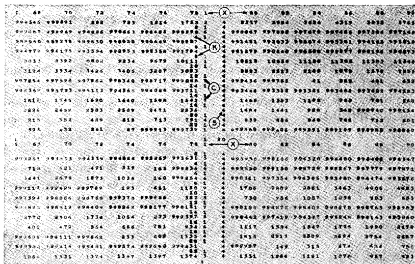
FIG. 5. Two-dimensional Fourier series. Sample first-step summation giving the coefficients of the sine and cosine terms of the second summation for z=0.068, 0.070, \dots, 0.090 .
