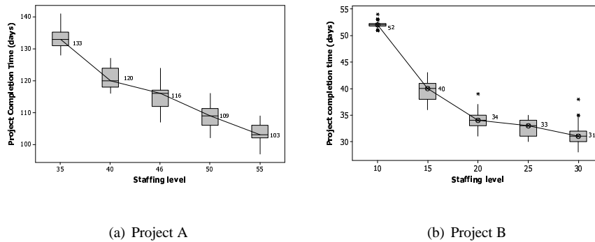
Figure 9. Boxplots of estimated project completion times for different staffing levels.
