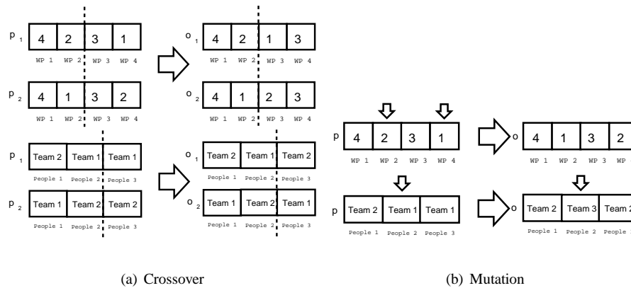
Figure 6. Crossover and mutation operators for WP ordering and developers allocation to teams.
