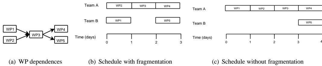
Figure 3. Example of fragmented schedule and of non-fragmented schedule with a higher completion time.
