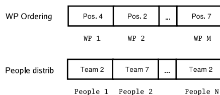
Figure 2. Solution representation.
