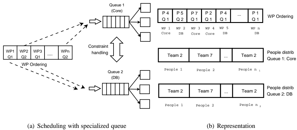
Figure 5. Schedule with specialized queues: (a) multi queue approach, and (b) representation.
