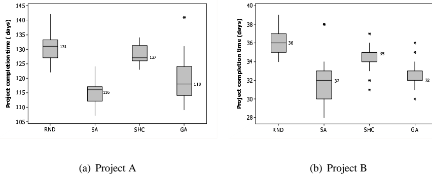
Figure 8. Boxplots of estimated project completion times for different algorithms.
