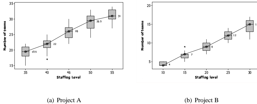
Figure 10. Boxplots of number of allocated teams for different staffing levels.
