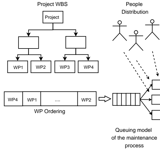
Figure 1. Project scheduling: the queuing model.
