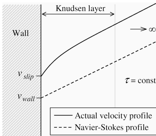
FIG. 1. Schematic of Kramer's problem: a gas in a half space, bounded by a planar wall, subject to a uniform and constant shear stress \tau . The Navier-Stokes solution with no-slip boundary condition (---) departs significantly from the actual velocity profile (—), and the velocity of the gas at the wall ( v_{slip} ) is different to the velocity of the wall itself ( v_{wall} ).
