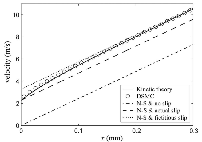
FIG. 2. Velocity profiles in Kramer's problem (planar wall at x=0 ). DSMC results for argon (o); kinetic theory (—); Navier-Stokes with fictitious slip (---); Navier-Stokes with actual slip (---); Navier-Stokes with no slip (· · ·). Values extracted from DSMC data: applied shear stress \tau=0.5 \text{ N m}^{-2} ; dynamic viscosity \mu=20.5 \times 10^{-6} \text{ N m}^{-2} \text{ s}^{-1} ; mean free path \lambda=118 \times 10^{-6} \text{ m} . For the equivalent DSMC calculation of Couette flow, the second wall is situated at x=1 \text{ mm} .
