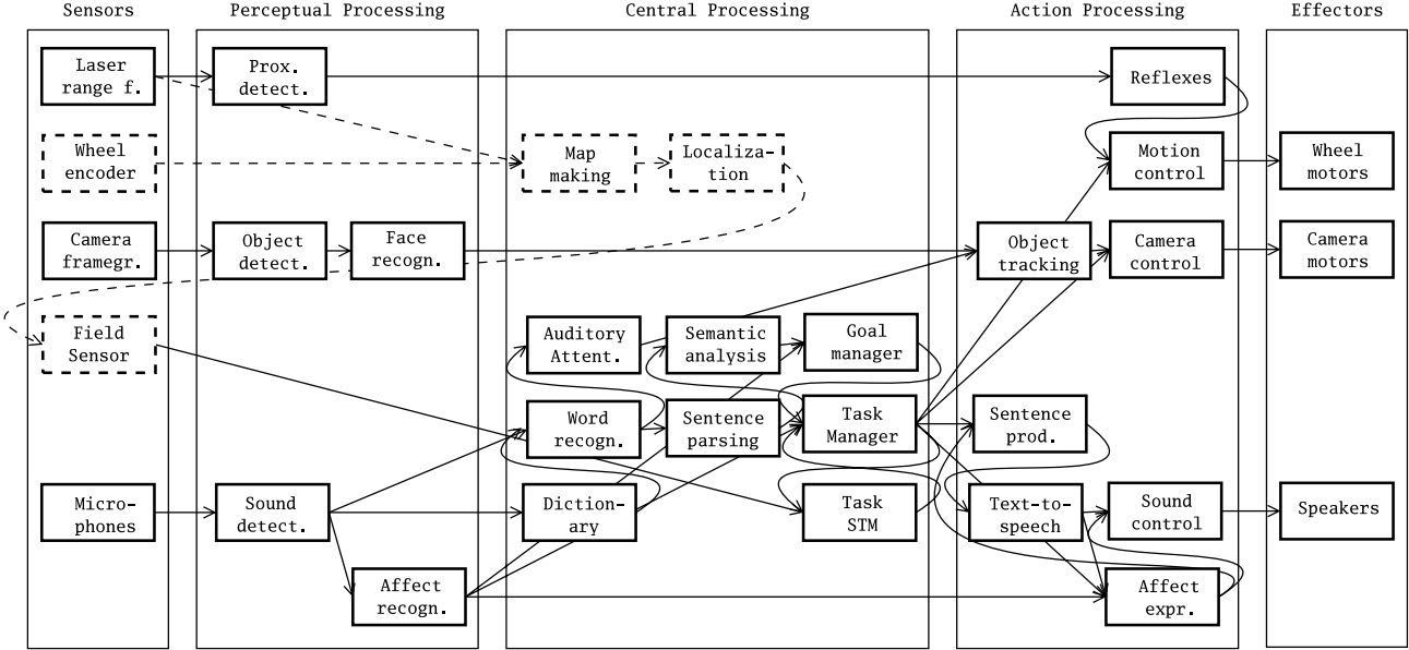
Figure 1: A partial view of the proposed DIARC robotic architecture for HRI consisting of only those components that were used in the experiment described in this paper. Boxes depict concurrently running components of varying complexity and arrows indicate the information flow through the architecture. Dashed items are related to the simulated field sensor, and are not part of the architecture per se (see the experiment description).
