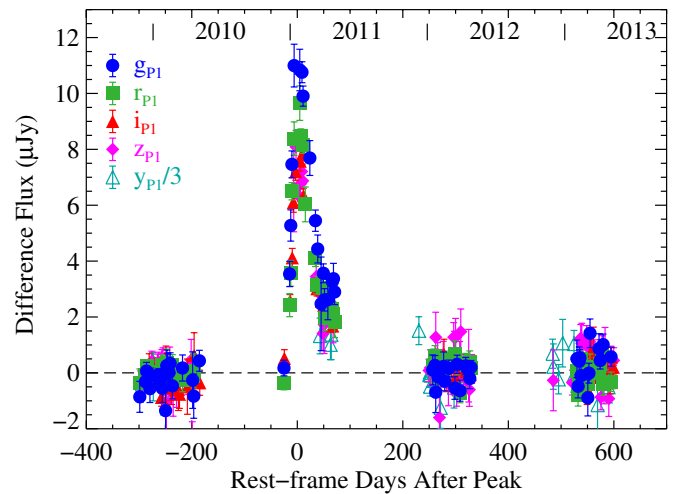
Figure 5. Long-term difference flux light curve of PS1-11af in five filters. The calendar years of observations are labeled across the top. The y_{p1} light curve has been divided by three for clarity because the observations are shallower than in the other bands so the typical scatter is larger. This light curve was constructed using a template image composed of an average of several of these same epochs of observation, which means that the zeropoint of the flux scale has an arbitrary constant offset level that we set to zero in the first year.
