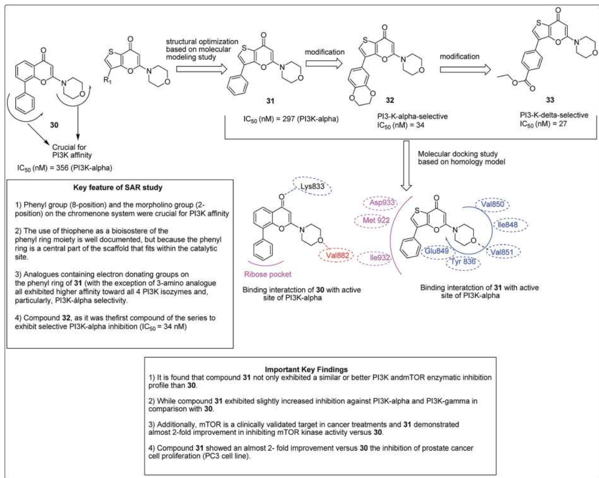
Fig. 5 5-Morpholino-7H-thieno[3,2-b]pyran-7-ones designed as next generation PI3K inhibitors along with SARs.
