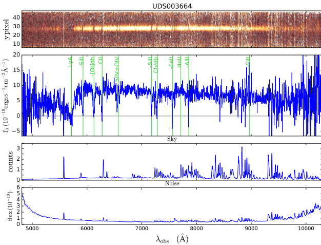
Fig. 9. From top to bottom : 2D spectrum, 1D extracted spectrum, sky counts, and rms noise of target VANDELS-UDS-003664. This object has an H -band magnitude of 23.1 and was selected in the category SFG. It was assigned a z_{\text{spec}} = 3.703 and Flag 4. The main spectral features (the \text{Ly}\alpha absorption and several interstellar absorption lines) are indicated in the 1D spectrum.
