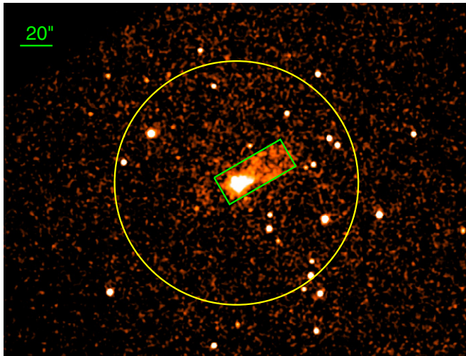
Figure 3. 0.5–7 keV image mosaic of the three Chandra observations (see Table 2). The green 47'' \times 19'' box marks the region used to extract the Chandra spectra, which includes the nuclear source plus a spectrally soft, conically shaped X-ray plume (Schurch et al. 2002; Done et al. 2003). The yellow circle ( 75'' radius) marks the NuSTAR source extraction region.
