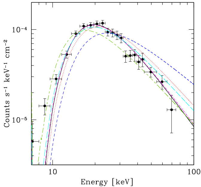
Figure 10. Spectrum obtained by subtracting the L state spectrum from the SH state spectrum (black solid points). The lines show the best-fit model allowing variations of: (a) normalization of the primary continuum (red dotted line); (b) photon index of the primary continuum (blue short dashed line); (c) absorbing column density of the primary continuum (olive short dashed-long dashed); (d) normalization and photon index of the primary continuum (black solid line); (e) normalization and absorbing column density of the primary continuum (cyan long-dashed line); (f) normalization, photon index, and absorbing column density of the primary continuum (magenta dotted-short dashed).
