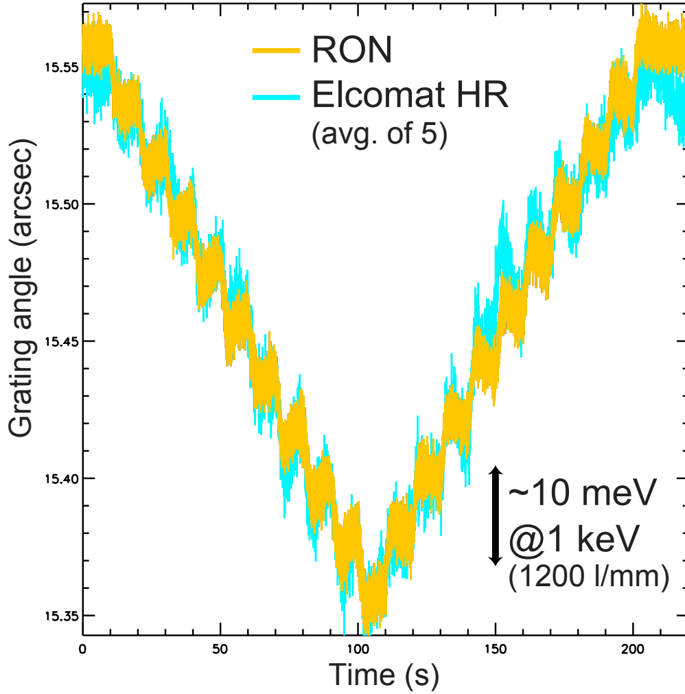
Figure 2: Mechanical performance of the rotational movement of the grating inside the PM/PG-U vessel of beamline P04 (branch 2). The curves showing the internally (RON) as well as externally (Elcomat HR) measured rotation are obtained by a stepwise rotation of the grating. Each step corresponds to 0.02 arcsec with an interval of 10 s between each of the consecutive steps. An arrow indicates the corresponding rotation of the 1200 l/mm grating for a 10 meV energy step at 1 keV photon energy.
