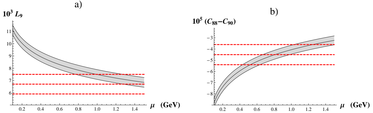
Figure 3: The R\chi T predictions (solid gray band) for the \chi PT \mathcal{O}(p^4) low-energy constant L_9(\mu) (a) and the \mathcal{O}(p^6) combination C_{88}(\mu) - C_{90}(\mu) (b) are compared to their large- N_C estimates (red dashed) for different values of the renormalization scale \mu . The error of the large- N_C estimate is given by the naive saturation scale uncertainty from Eq. (22).
