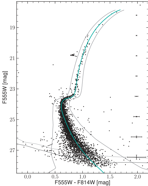
Figure 2. Observed CMD of Pal 4. Error bars on the right represent the photometric errors derived from artificial star tests. The grey lines at the faint end represent the 80 per cent (light grey) and 50 per cent (dark grey) completeness contours. The isochrone (cyan line) corresponds to an age of 11 Gyr, a metallicity of [\text{Fe}/\text{H}] = -1.41 dex and an \alpha -enhancement of [\alpha/\text{Fe}] = +0.4 dex, shifted to the cluster’s distance of 20.06 mag at a reddening of E(B - V) = 0.023 mag. Thin grey curves to the left and to the right of the isochrone represent the colour limits used for our analysis of the cluster’s mass function (see Section 4).
