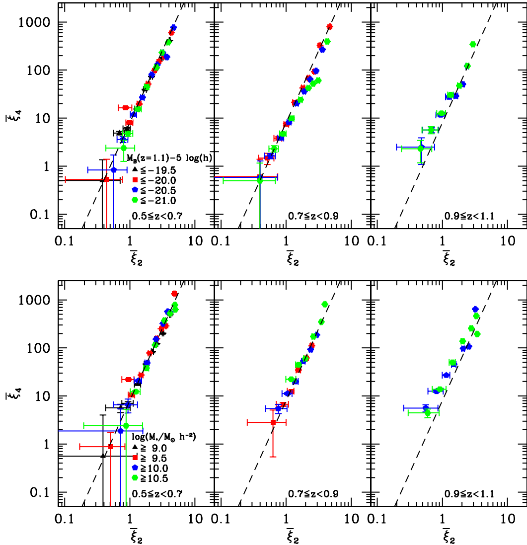
Fig. 8. Scaling relation of the volume-averaged two and four-point correlations as a function of the B absolute luminosity ( upper panels ) and stellar mass ( lower panels ). The limits of the subsamples in absolute magnitude and stellar mass are shown in the left upper and lower panels (symbols and colours are the same as in Fig. 4). The dashed line represents the scaling relation \log_{10}(\xi_3) = 3 \log_{10}(\xi_2) + \log_{10}(8) .
