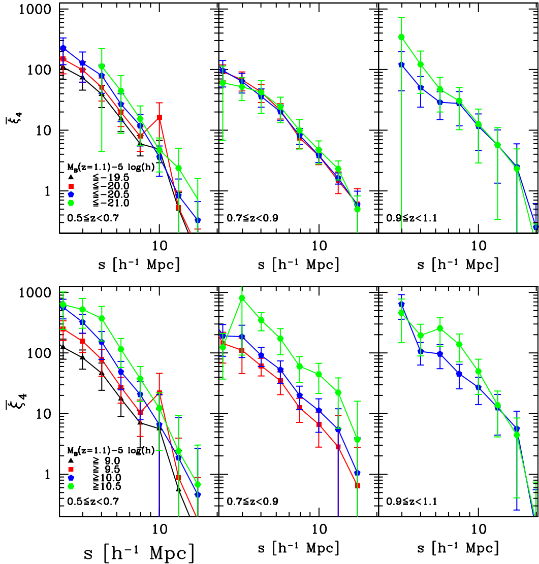
Fig. 6. Volume-averaged four-point correlation functions as a function of the B absolute luminosity ( upper panels ) and stellar mass ( lower panels ). The limits of the subsamples in absolute magnitude and stellar mass are shown in the left upper and lower panels (symbols and colours are the same as in Fig. 4).
