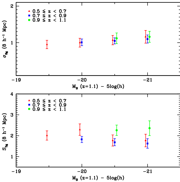
Fig. 12. \sigma_{8g} (upper panel) and S_{3g} at R = 8 h^{-1} Mpc (lower panel) as a function of galaxy luminosity for the three redshift bins. Red triangles: 0.5 \leq z < 0.7 ; blue squares: 0.7 \leq z < 0.9 ; green hexagons: 0.9 \leq z < 1.1 . For better visibility, points corresponding to different redshifts are slightly shifted in magnitude.
