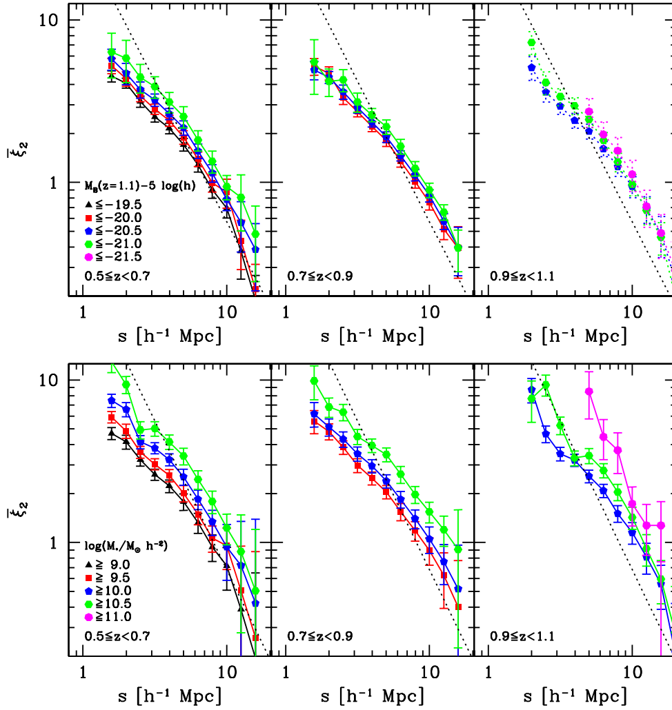
Fig. 4. Volume-averaged two-point correlation functions \bar{\xi}_2 as a function of the B absolute luminosity ( upper panels ) and stellar mass ( lower panels ). The limits of the subsamples in absolute magnitude and stellar mass are shown in the left upper and lower panels . Black triangles: M_B(z = 1.1) - 5 \log(h) \leq -19.5 ( \log(M_*/M_\odot h^{-2}) \geq 9.0 M_\odot ); red squares: M_B(z = 1.1) - 5 \log(h) \leq -20.0 ( \log(M_*/M_\odot h^{-2}) \geq 9.5 M_\odot ); blue pentagons: M_B(z = 1.1) - 5 \log(h) \leq -20.5 ( \log(M_*/M_\odot h^{-2}) \geq 10.0 M_\odot ); green hexagons: M_B(z = 1.1) - 5 \log(h) \leq -21.0 ( \log(M_*/M_\odot h^{-2}) \geq 10.5 M_\odot ); magenta heptagons: M_B(z = 1.1) - 5 \log(h) \leq -21.5 ( \log(M_*/M_\odot h^{-2}) \geq 11.0 M_\odot ). Dotted lines: real-space \bar{\xi}_2 for the M_B(z = 1.1) - 5 \log(h) \leq -20.5 ( \log(M_*/M_\odot h^{-2}) \geq 10.0 M_\odot ) subsamples in the redshift bin [0.5, 0.7] , predicted from the power-law fit of \xi_2 in Marulli et al. (2013).
