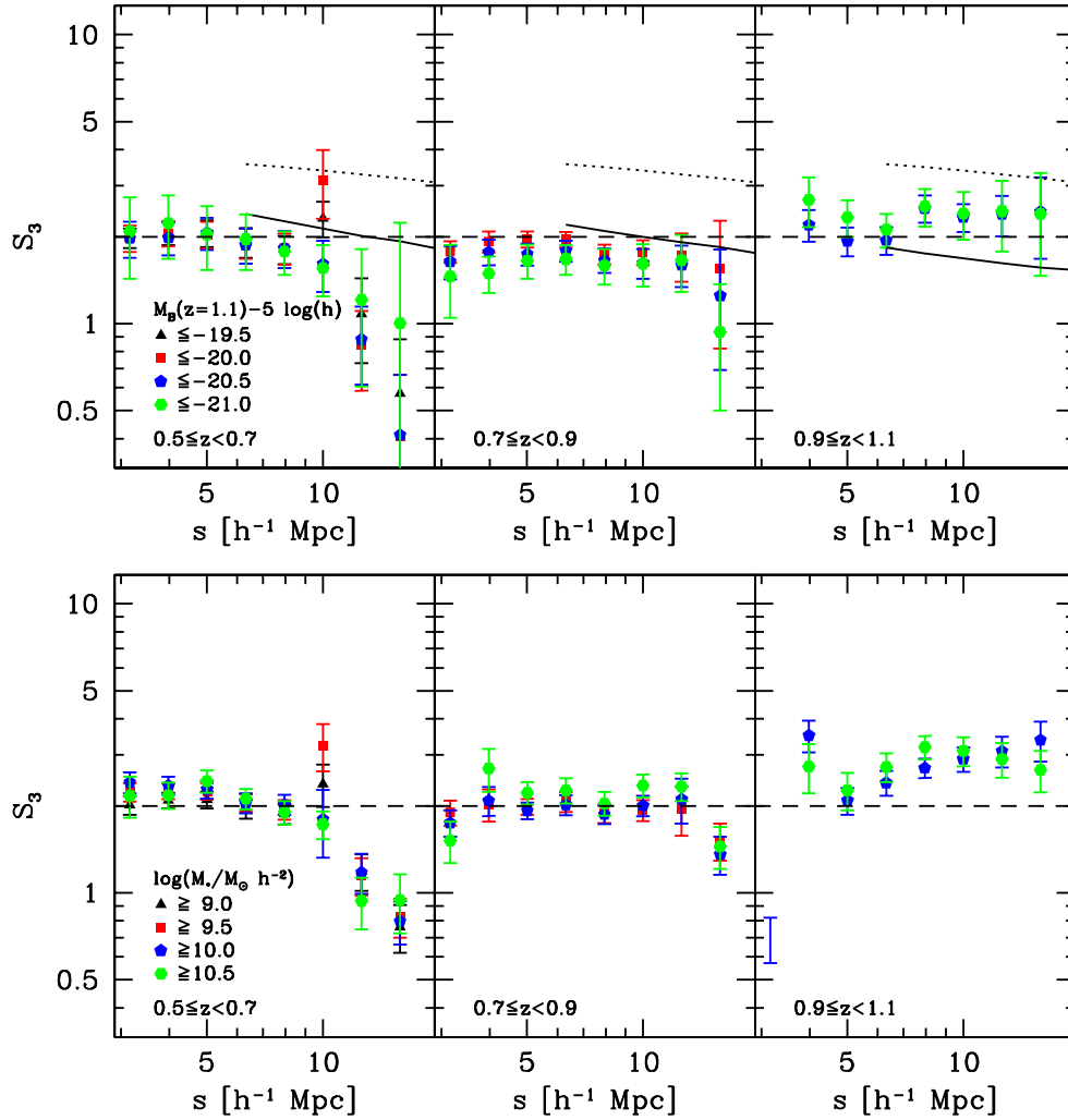
Fig. 9. Normalized skewness S_3 as a function of the B absolute luminosity ( upper panels ) and stellar mass ( lower panels ). The limits of the subsamples in absolute magnitude and stellar mass are shown in the left upper and lower panels (symbols and colours are the same as in Fig. 4). We note that black points corresponding to galaxies with M < -19.50 or M_* \geq 9.0 M_\odot are only plotted for the first redshift bin ( [0.5, 0.7] ), but most of them are not visible as they lie below the points of the other samples. The dashed line corresponds to S_3 = 2 . In the top panels , the dotted line is the prediction from second-order perturbation theory for the matter distribution in real space; the solid line is the prediction of S_3 for galaxies with M_B(z = 1.1) - 5 \log(h) \leq -20.5 (to be compared to blue pentagons); it was obtained from the matter values, converted to redshift space and divided by the corresponding linear bias factor.
