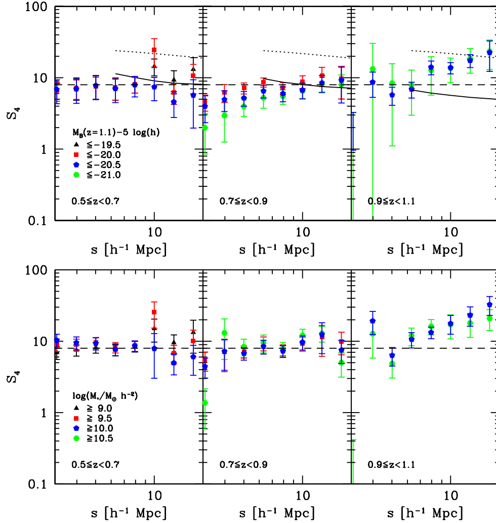
Fig. 10. Normalized skewness S_4 as a function of the B absolute luminosity ( upper panels ) and stellar mass ( lower panels ). The limits of the subsamples in absolute magnitude and stellar mass are shown in the left upper and lower panels (symbols and colours are the same as in Fig. 4). We note that black points corresponding to galaxies with M < -19.50 or M_* \geq 9.0 M_\odot are only plotted for the first redshift bin ( [0.5, 0.7] ), but most of them are not visible as they lie below the points of the other samples. The dotted line is the prediction from second-order perturbation theory for the matter distribution in real space; the dashed line corresponds to S_4 = 8 . In the top panels , the dotted line is the prediction from second-order perturbation theory for the matter distribution in real space; the solid line is the prediction of S_4 for galaxies with M_B(z = 1.1) - 5 \log(h) \leq -20.5 (to be compared to blue pentagons): it was obtained from the matter values, converted to redshift space and divided by the corresponding linear bias factor.
