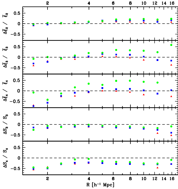
Fig. 2. Fractional difference of the average \bar{\xi}_2 , \bar{\xi}_3 , \bar{\xi}_4 , S_3 and S_4 (from top to bottom) for the same set of mock catalogues as defined in Fig. 1, i.e. with 100% sampling rate and without gaps, and with sampling rate and gaps as in VIPERS. The subsamples are limited at M_B(z = 1.1) - 5 \log(h) \leq -20.5 . Red triangles: 0.5 \leq z < 0.7 ; blue squares: 0.7 \leq z < 0.9 ; green hexagons: 0.9 \leq z < 1.1 .
