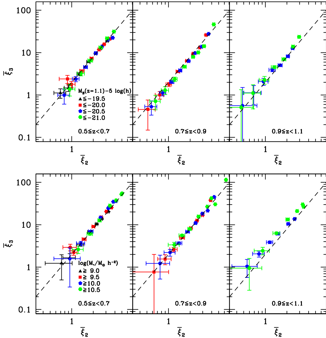
Fig. 7. Scaling relation of the volume-averaged two- and three-point correlations as a function of the B absolute luminosity ( upper panels ) and stellar mass ( lower panels ). The limits of the subsamples in absolute magnitude and stellar mass are shown in the left upper and lower panels (symbols and colours are the same as in Fig. 4). The dashed line represents the scaling relation \log_{10}(\bar{\xi}_3) = 2 \log_{10}(\bar{\xi}_2) + \log_{10}(2) .
