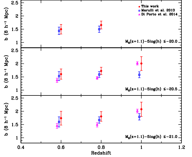
Fig. 13. Linear bias b as a function of redshift. Top panel: M_B \leq -20.0(z = 1.1) + 5 \log(h) ; middle panel: M_B \leq -20.5(z = 1.1) + 5 \log(h) ; bottom panel: M_B \leq -21.0(z = 1.1) + 5 \log(h) . Red hexagons: our estimates of b = \sigma_{8g}/\sigma_{8m} . Blue squares: estimates of Marulli et al. (2013). Magenta triangles: Di Porto et al. (2014).
